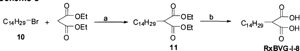
Scheme 8
