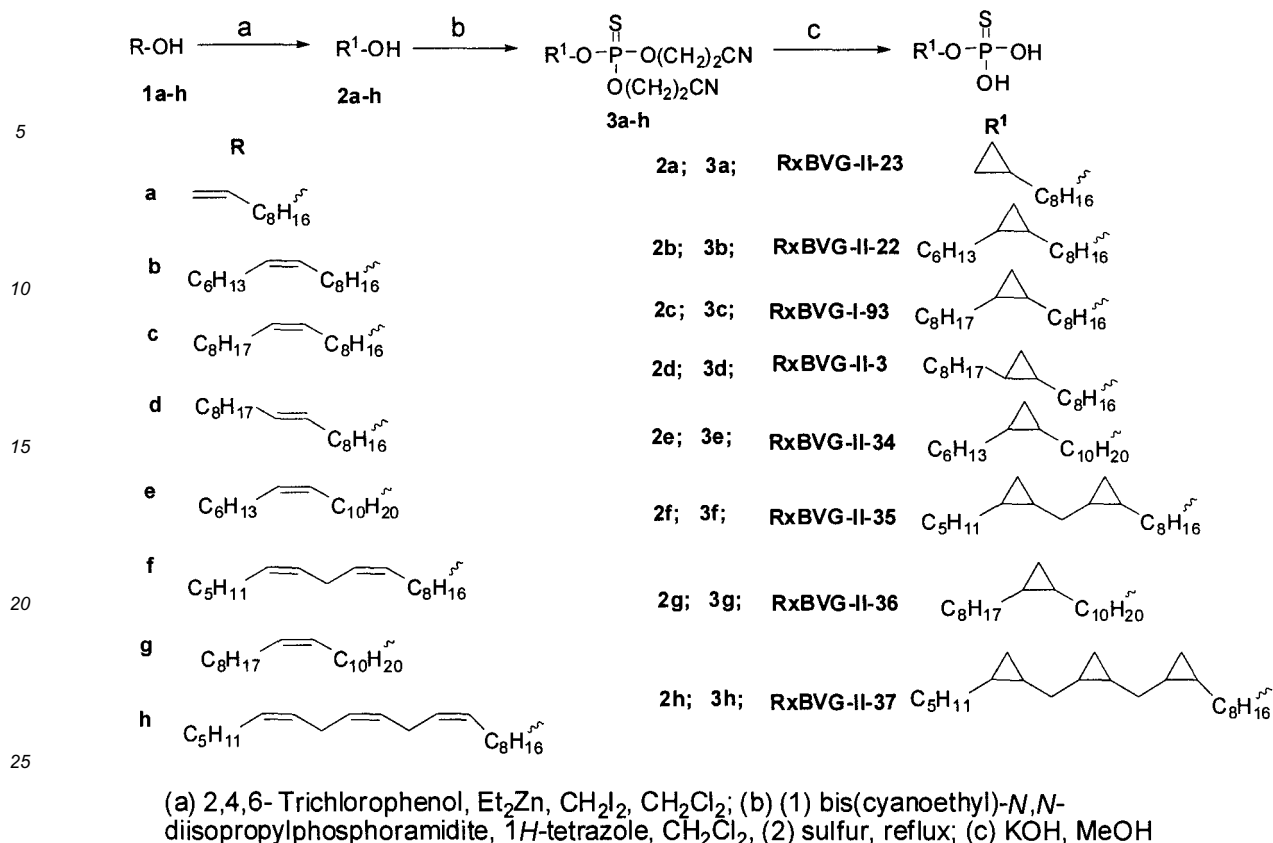
Scheme 5
