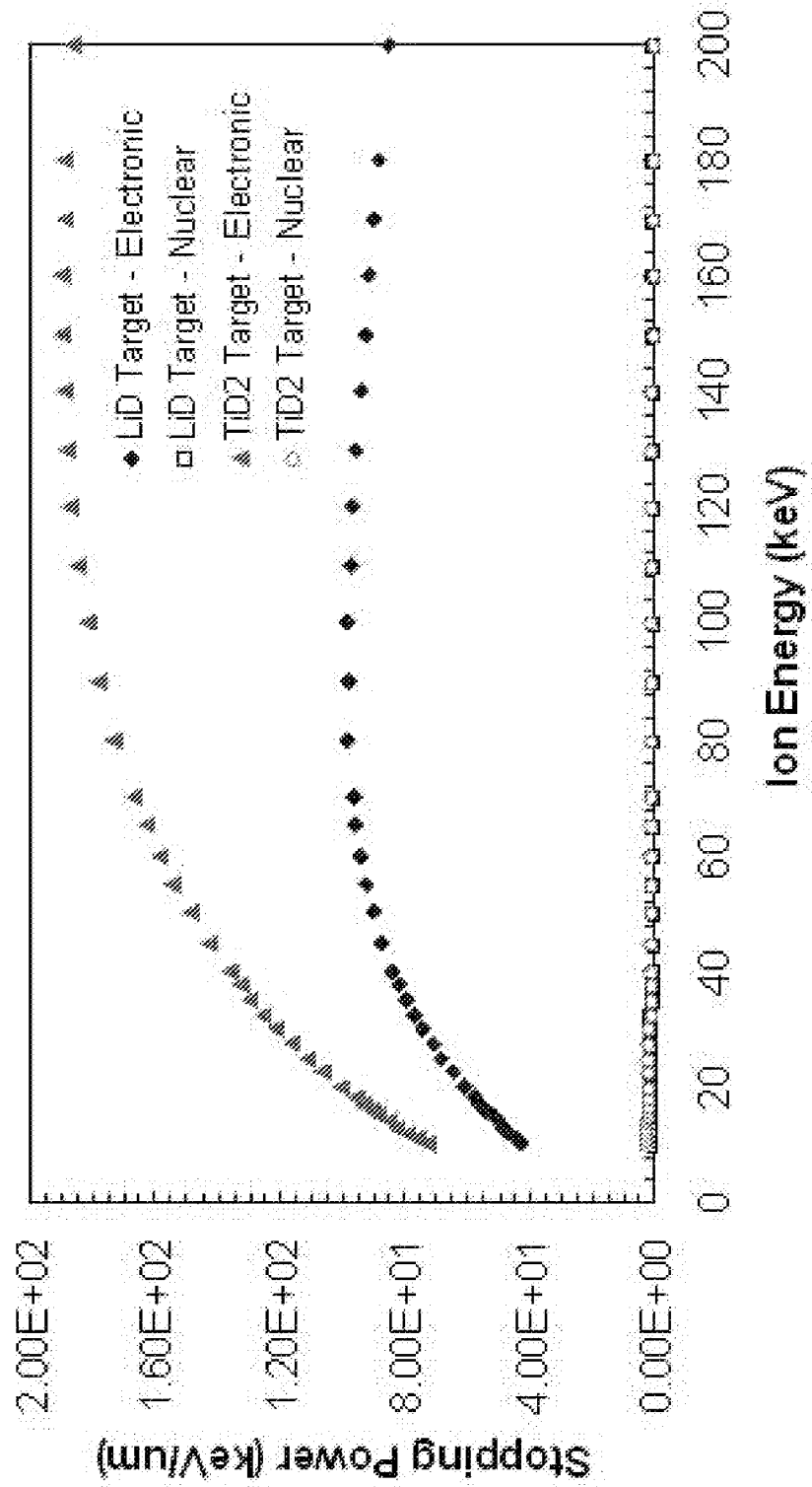
FIG. 12 Comparison of Stopping of Energetic Deuterons in LiD and TiD 2 As calculated by the SRIM package
