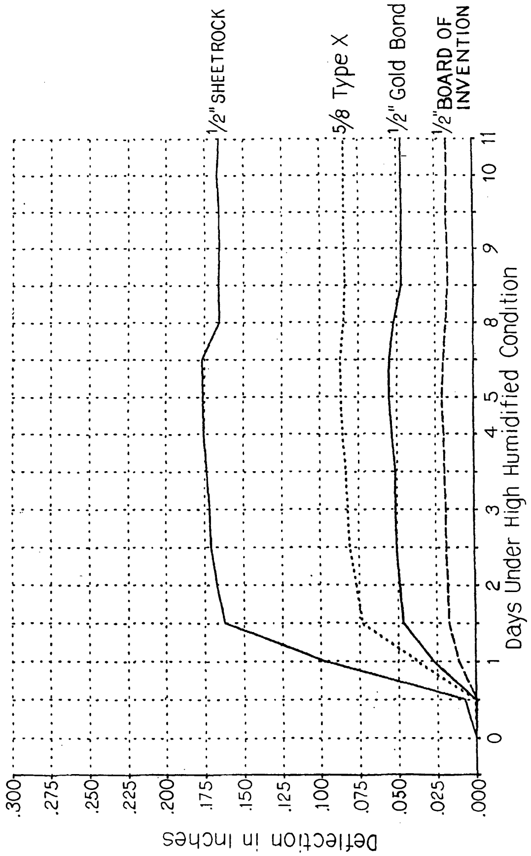
FIG. 3 F2100 Ceiling Sag Comparison
