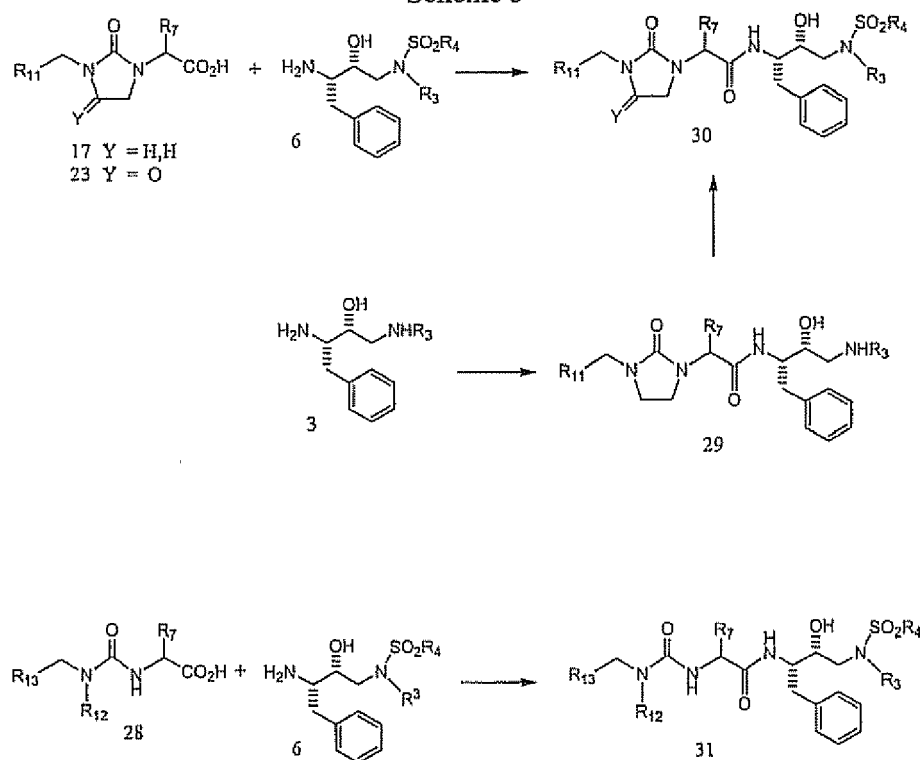
Scheme 5
