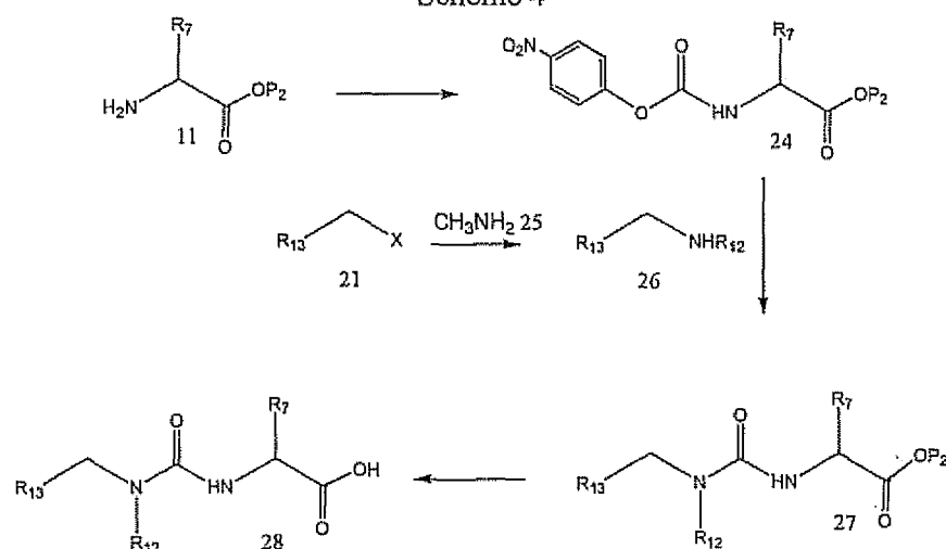
Scheme 4
