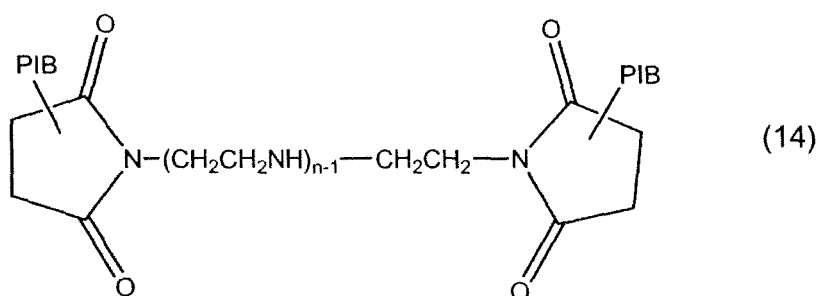
[Chemical Formula 7]
