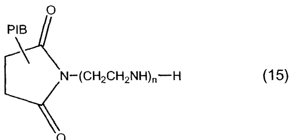
[Chemical Formula 8]
