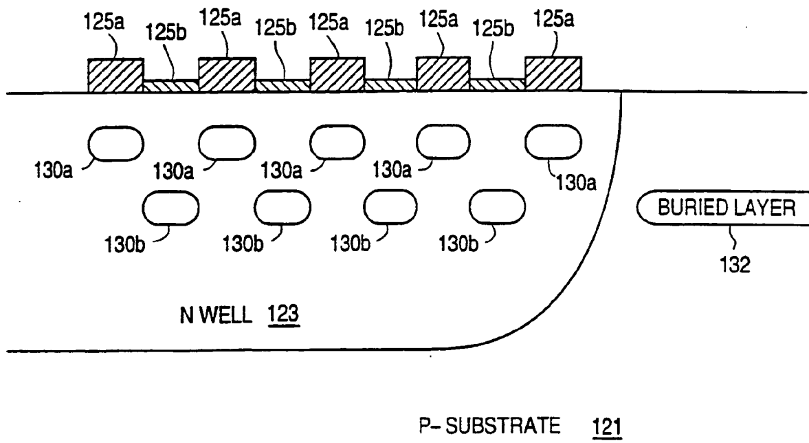
FIG. 11d
