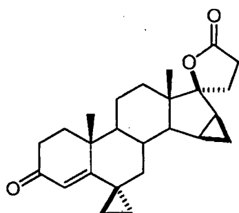
IVa: R_7, R_8 = \text{H}
