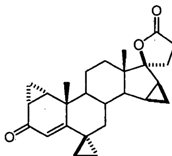
IVc: R_7, R_8 = \alpha\text{-CH}_2 \text{ bridge}
