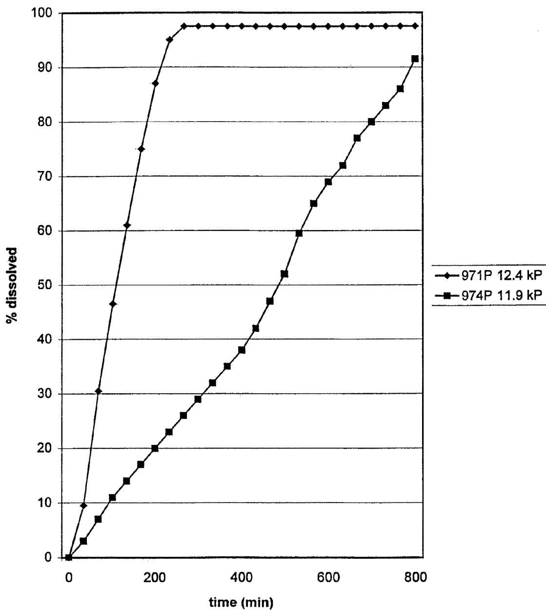
Figure 13: 5% Carbopol 971P NF and Carbopol 974P-NF controlled release over 12 hours
