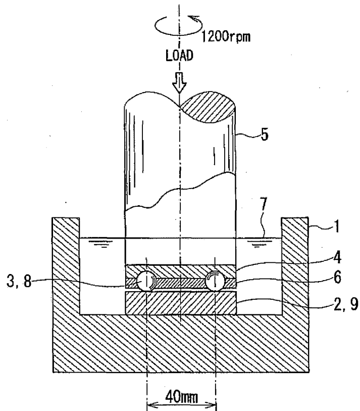
THRUST TYPE ROLLING WEAR TESTING APPARATUS
