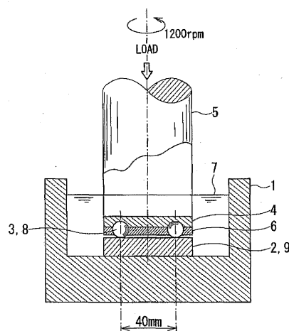
THRUST TYPE ROLLING WEAR TESTING APPARATUS
