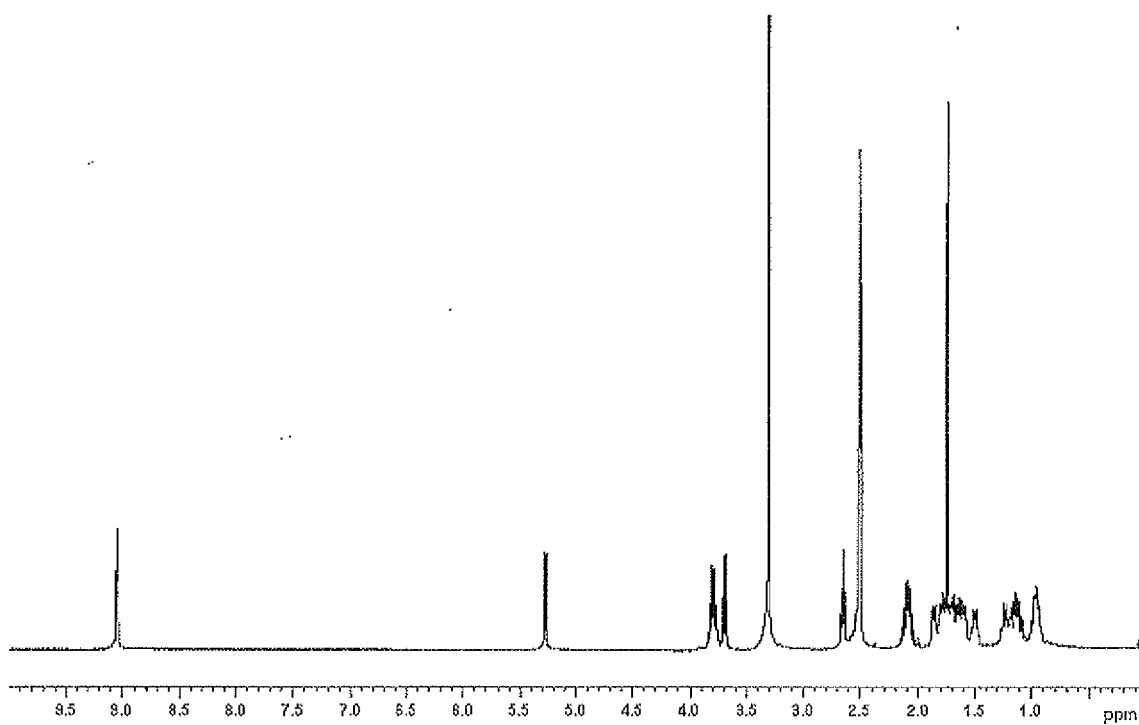
FIG. 5. 1 H NMR spectrum of compound of Formula II-4.
