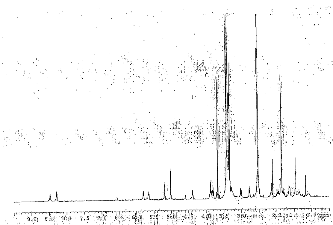
Fig. 33: ^1\text{H} -NMR of the compound of formula II-51
