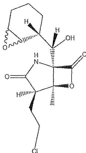
Formulae II-5A and II-5B
