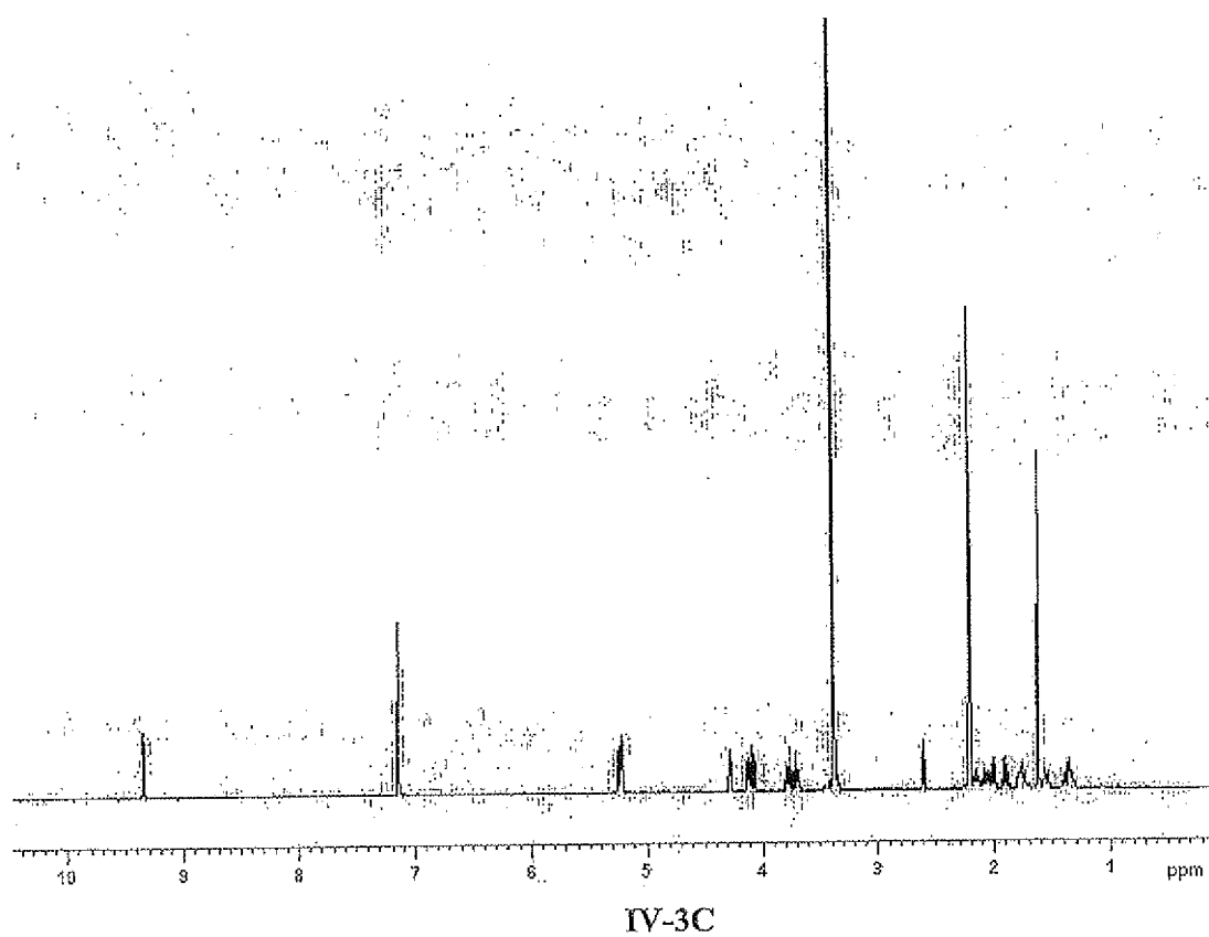
Figure 22. ^1\text{H} NMR spectrum of the compound of Formula IV-3C in \text{C}_6\text{D}_6/\text{DMSO-d}_6 .
