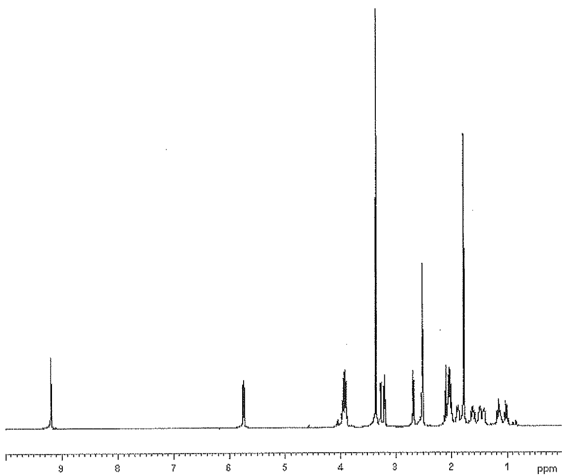
FIG. 7 ^1\text{H} NMR spectrum of compound of Formula II-5A.
