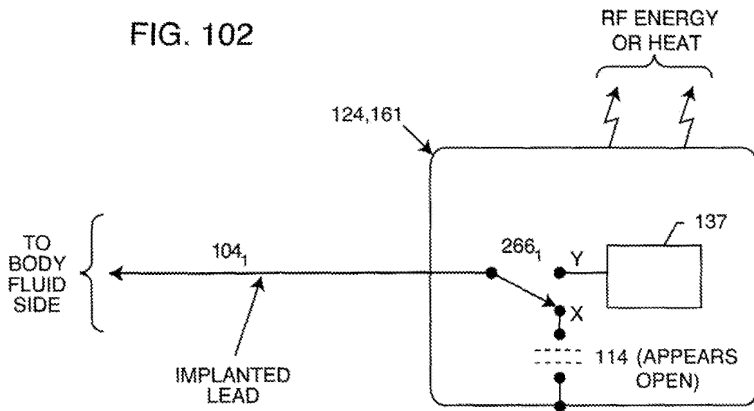
MRI PULSED RF (HIGH) FREQUENCY MODEL
