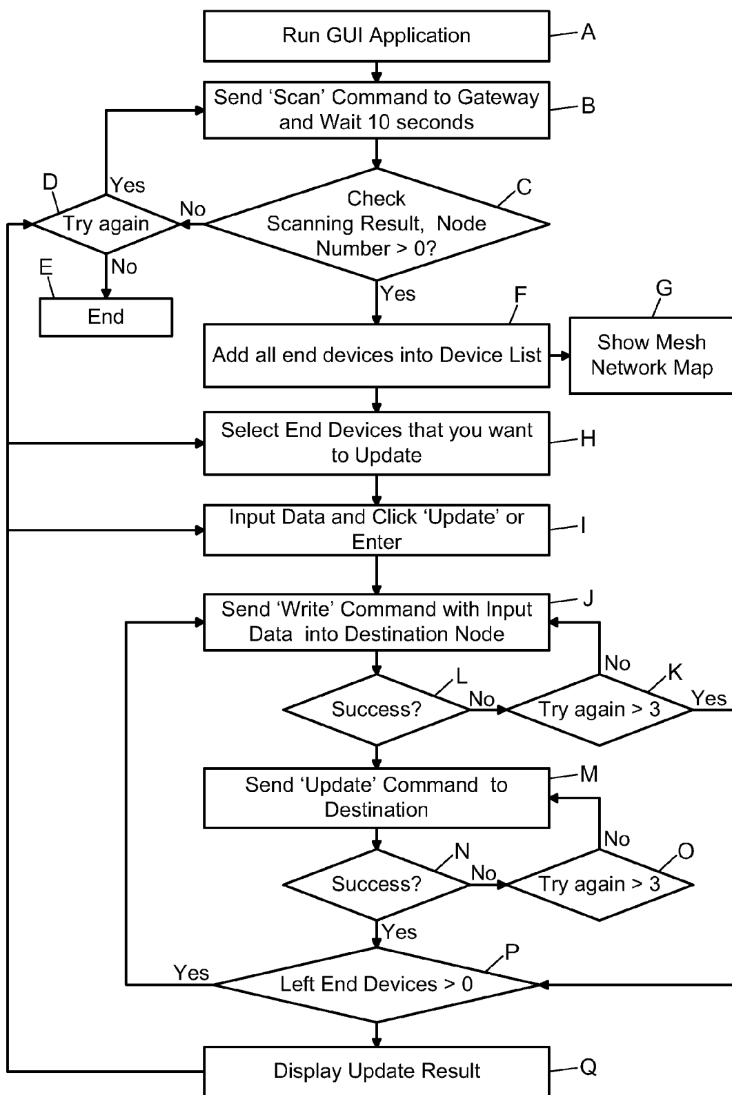
GUI Flow Chart
