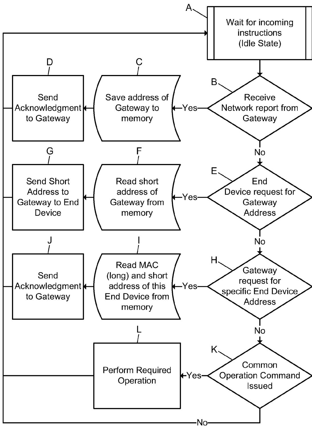
Network Coordinator Firmware Flowchart
