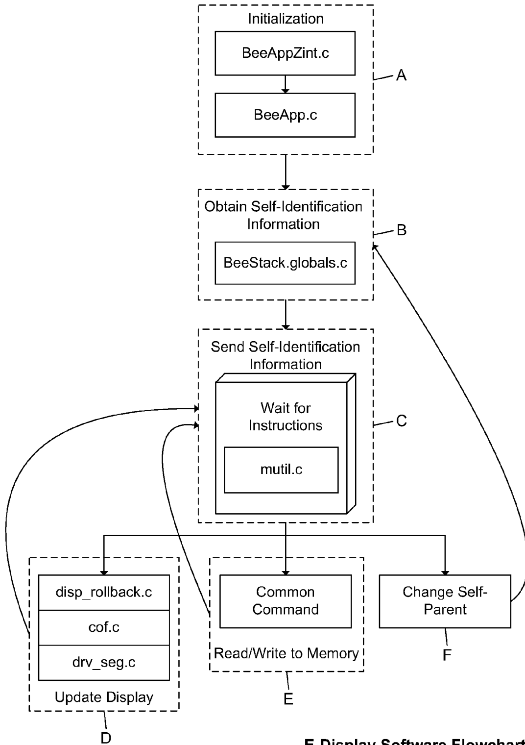
E-Display Software Flowchart
