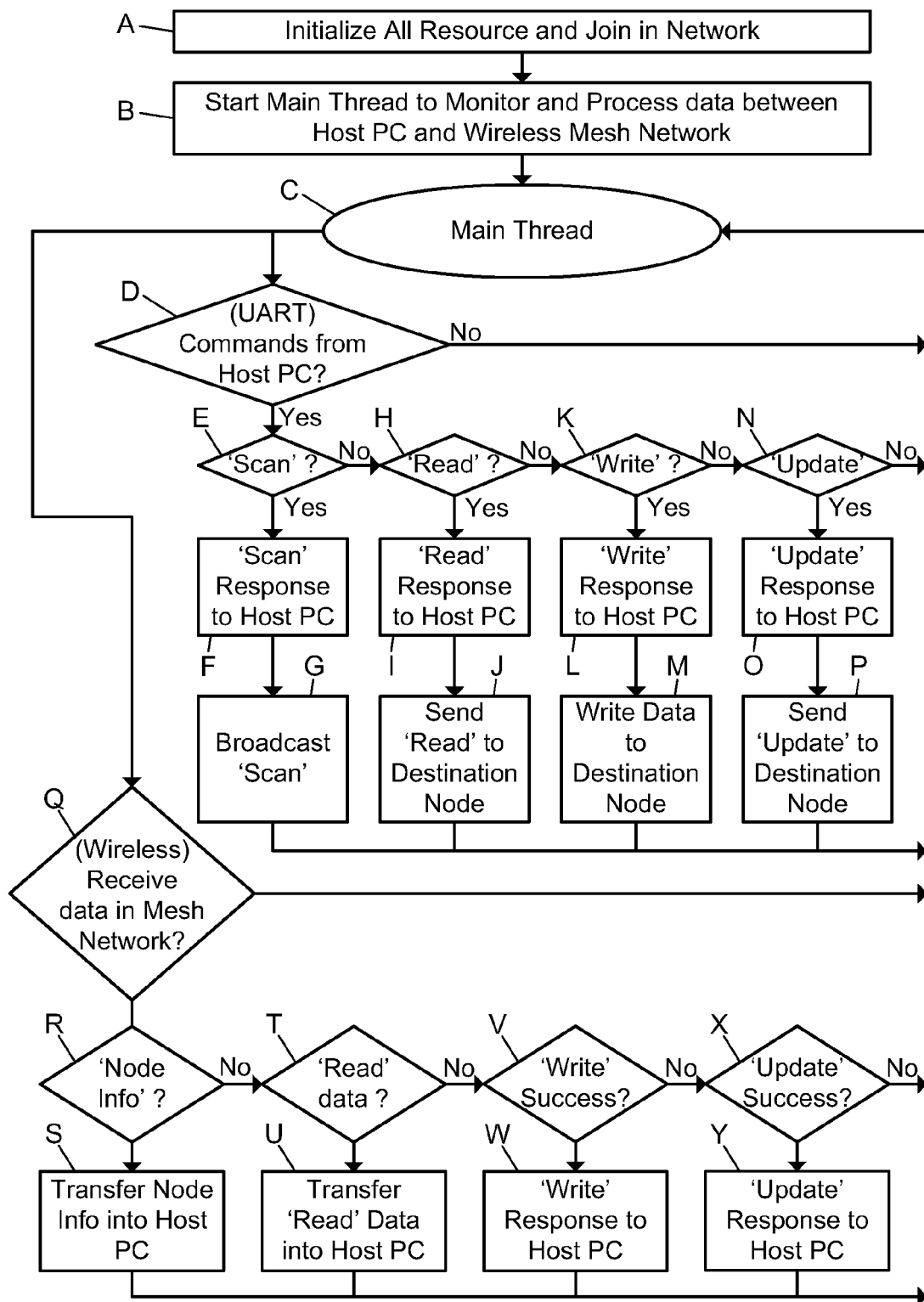
Gateway Firmware Flowchart
