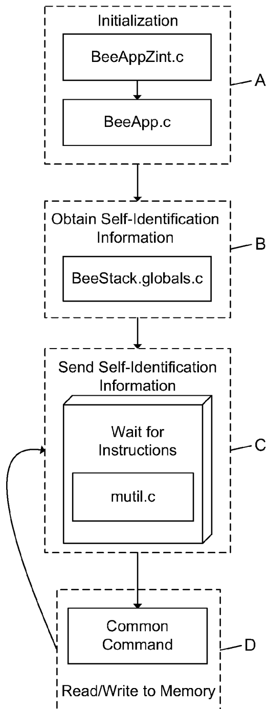
Coordinator Software Flowchart
