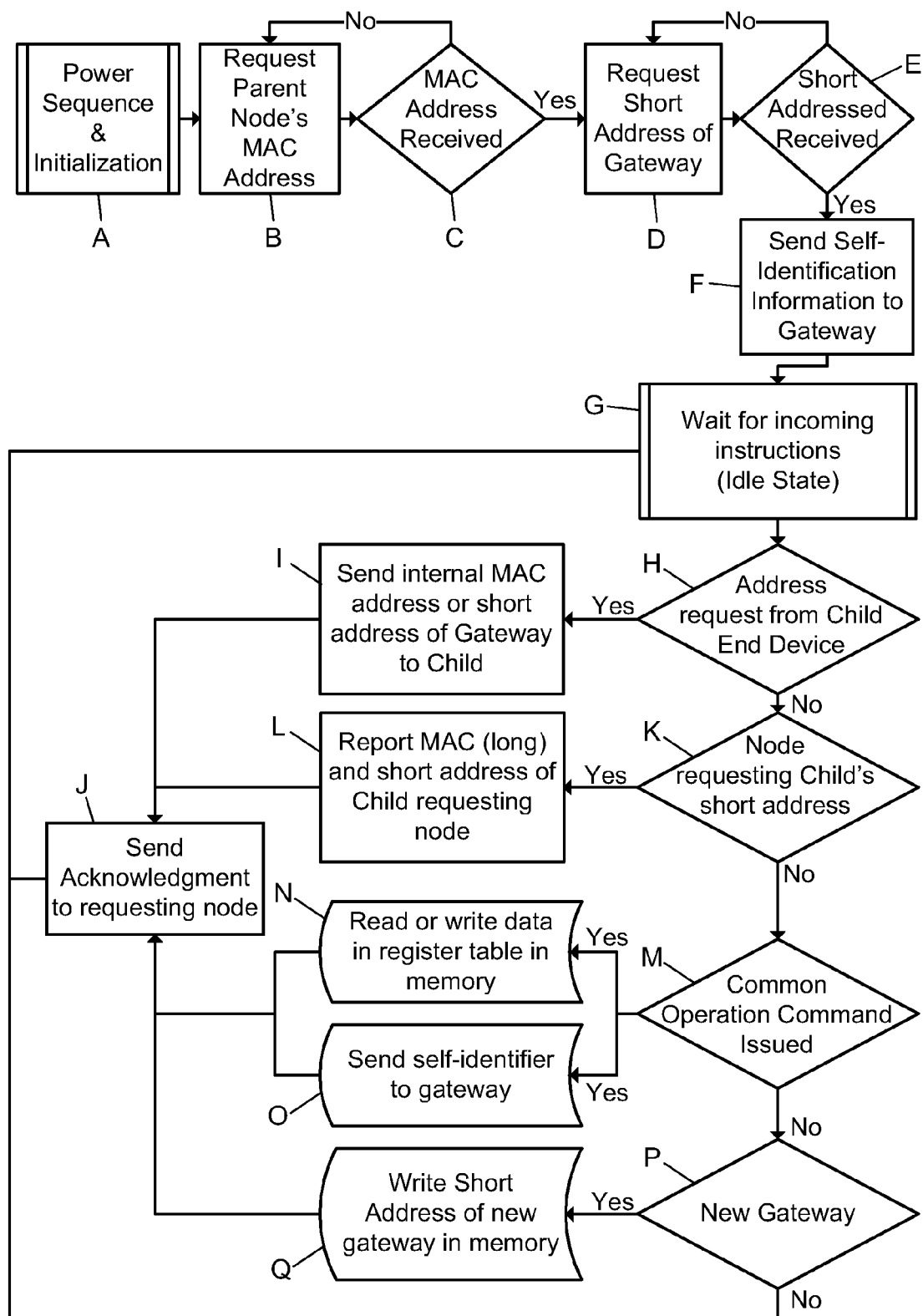
Zigbee Router Firmware Flowchart FIG. 8G
