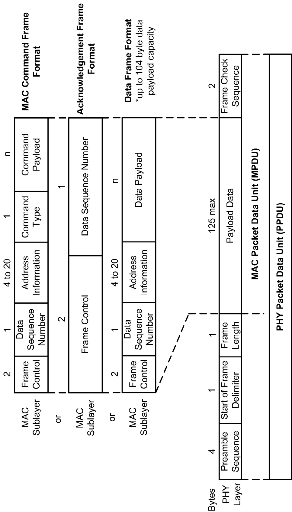
802.15.4 Packet Structures
