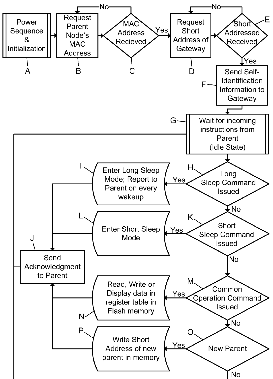
Zigbee End Device (E-Display) Firmware Flowchart
