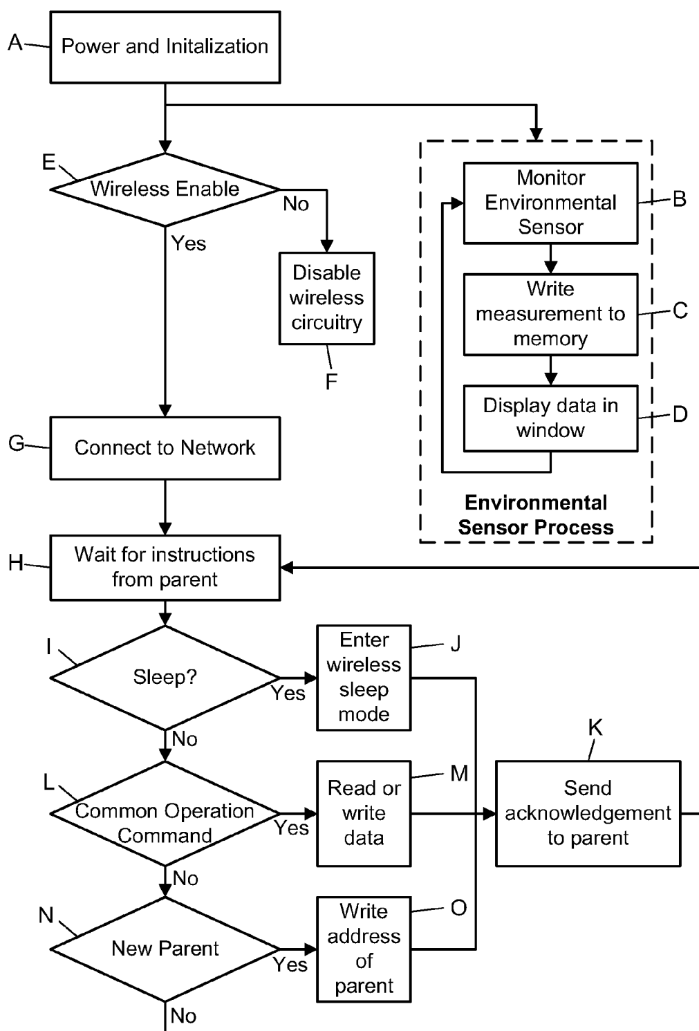
Operational Flowchart for Wireless E-Display Sensor
