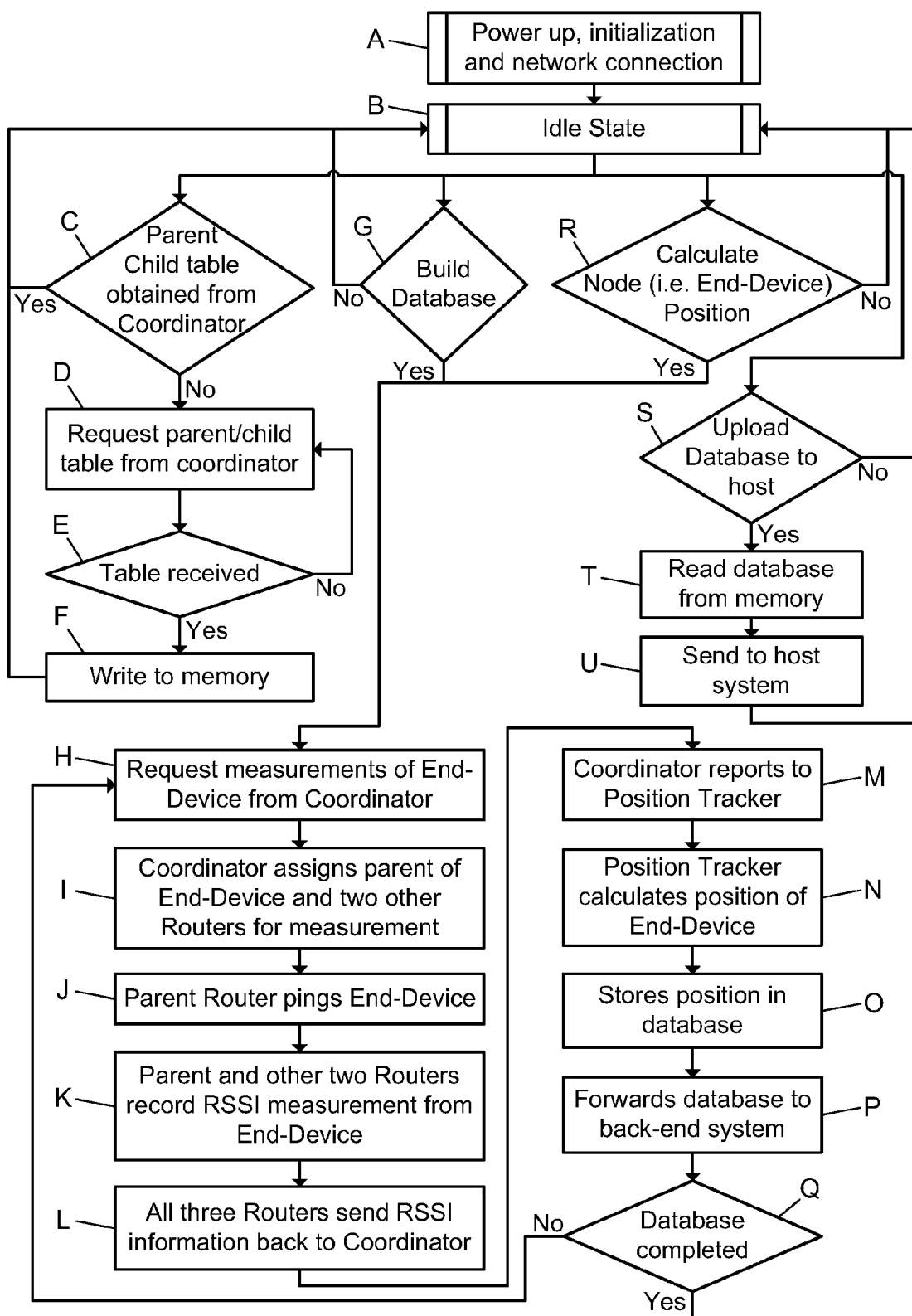
Position Tracking Module Flowchart
