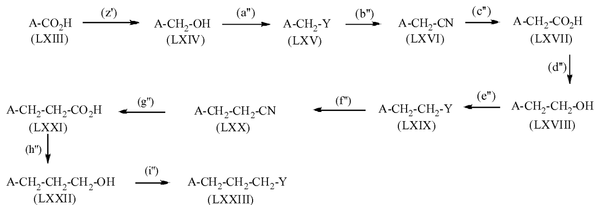
Reaction Scheme 12
