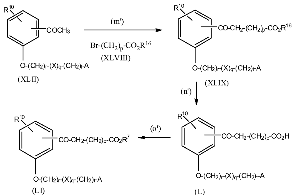
Reaction Scheme 6
