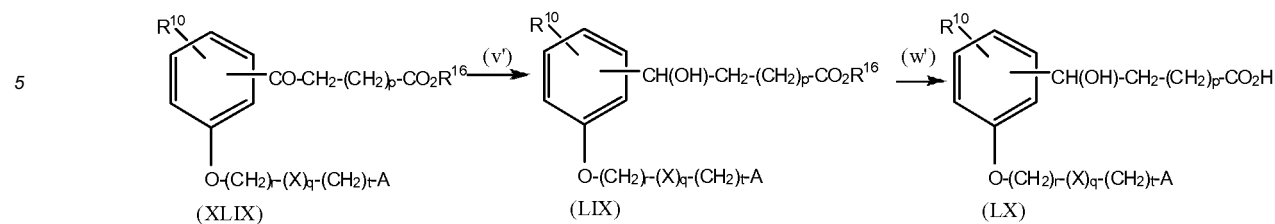
Reaction Scheme 10
