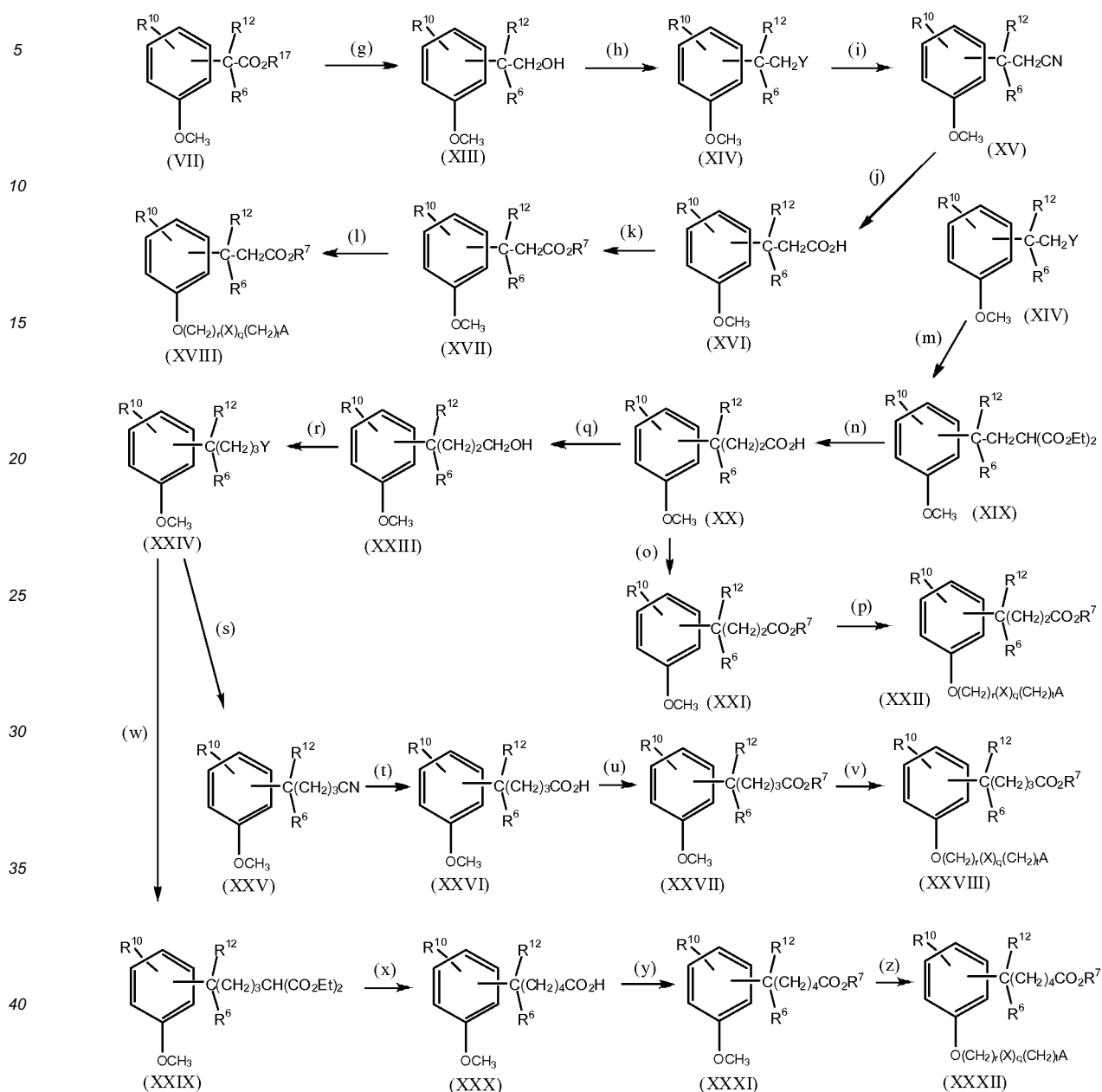
Reaction Scheme 2
