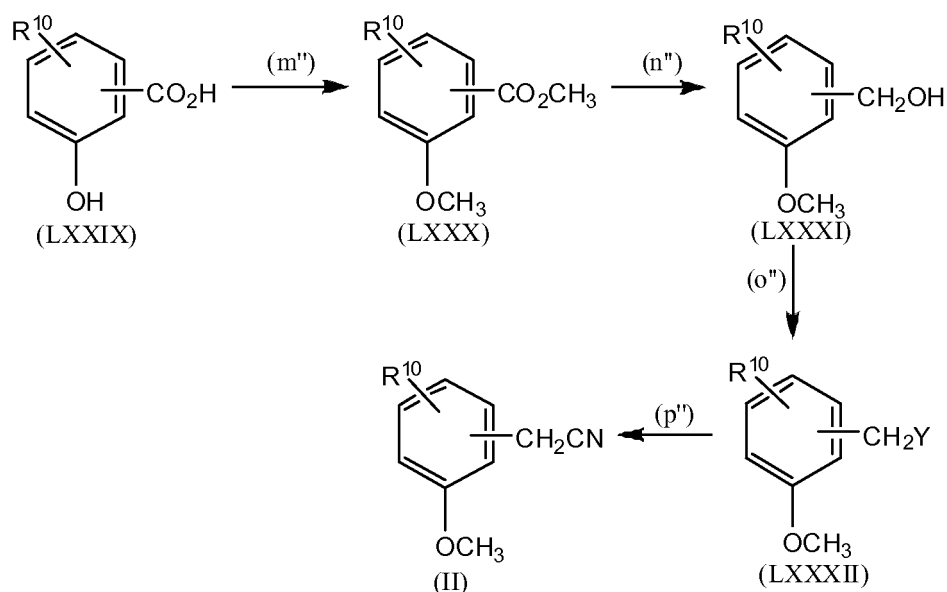
Reaction Scheme 14
