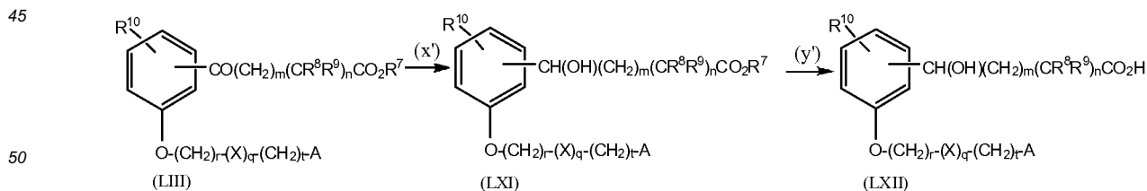
Reaction Scheme 11
