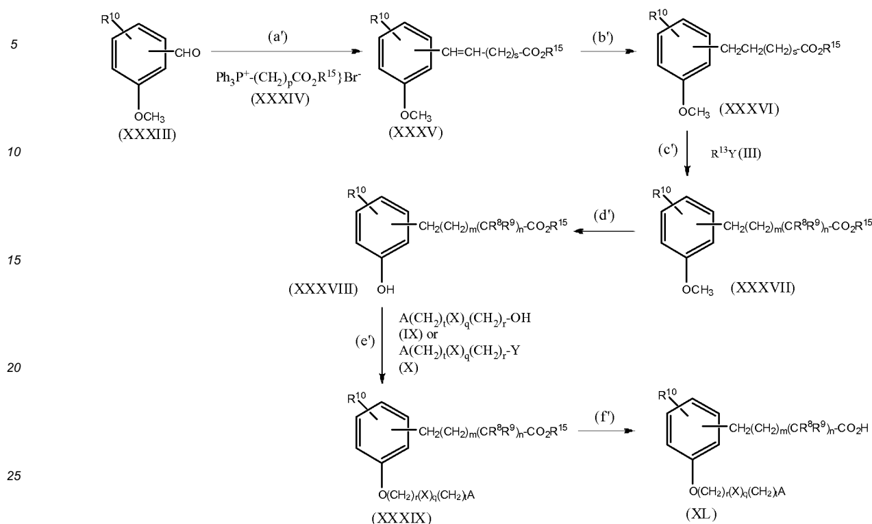
Reaction Scheme 3
