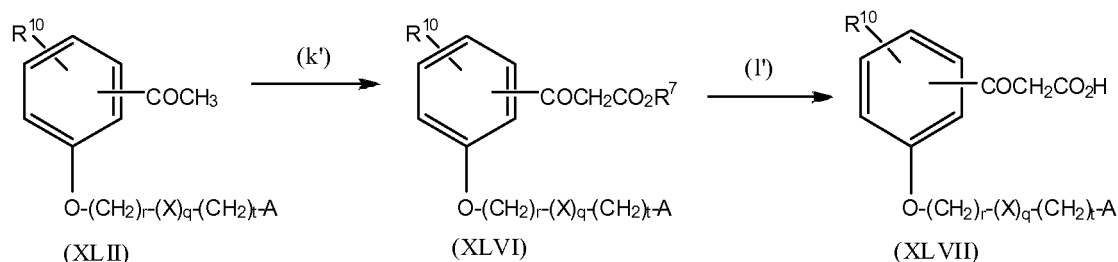
Reaction Scheme 5
