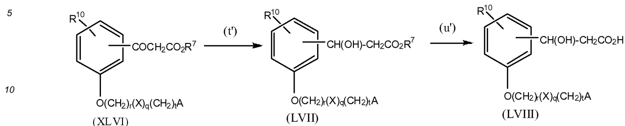
Reaction Scheme 9
