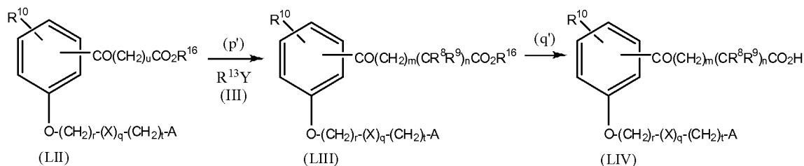
Reaction Scheme 7
