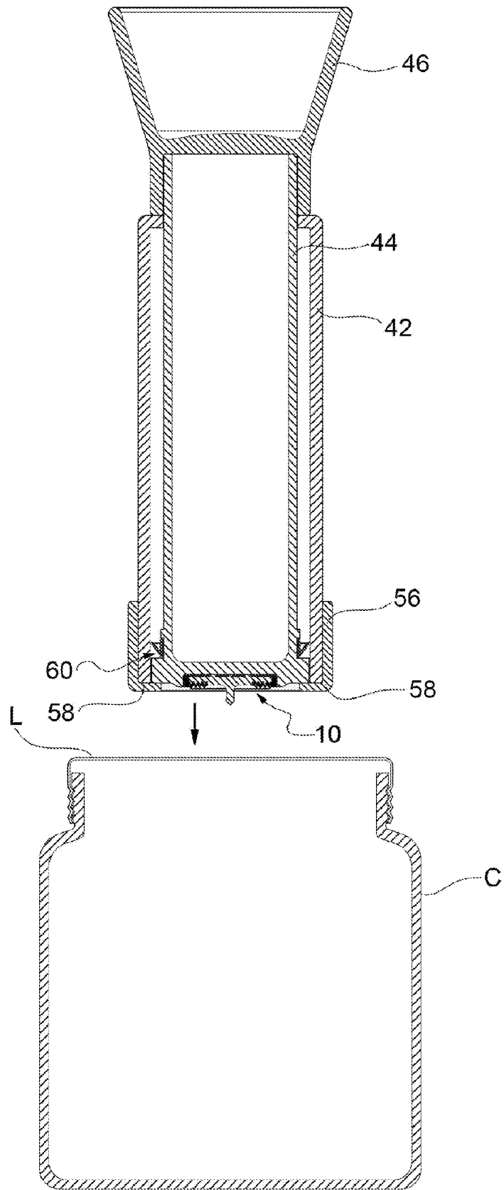
FIG.3d
