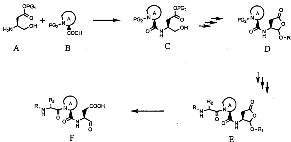
Scheme I. General scheme for the preparation of E and F
