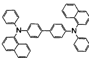
Compound 3
