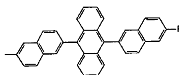
Compound 41
