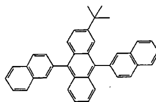
Compound 39
