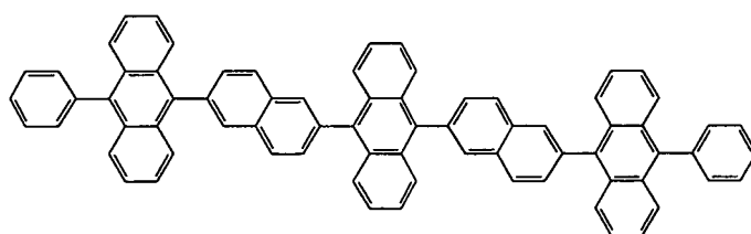
(Compound 38).
