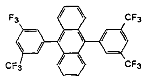
Compound 12
