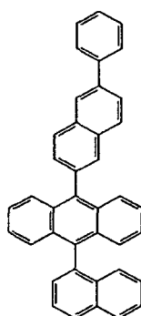
Compound 59
