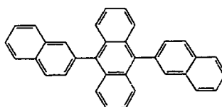
Compound 26
