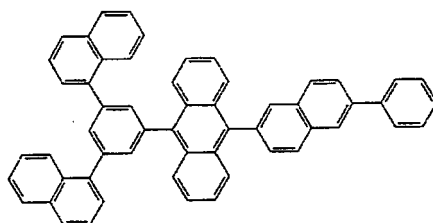
Compound 47
