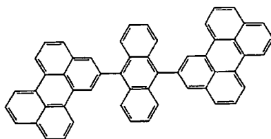
Compound 35
