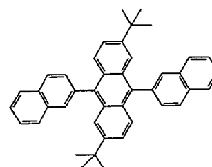
Compound 40
