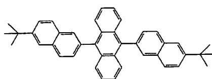
Compound 27
