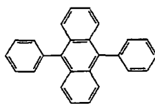
Compound 5
