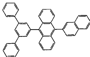
Compound 50
