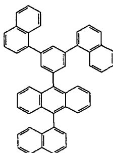
Compound 54
