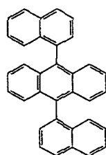
Compound 44
