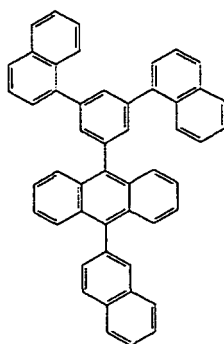
Compound 55
