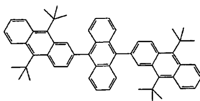
Compound 33
