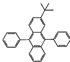
Compound 6
