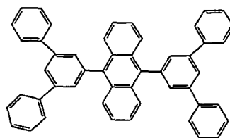
Compound 14
