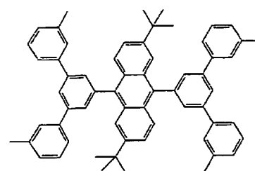
Compound 16
