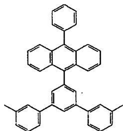
Compound 46
