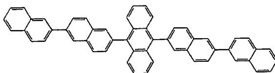
Compound 36
