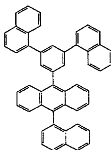
Compound 57
