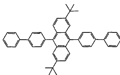
Compound 11
