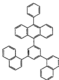
Compound 53
