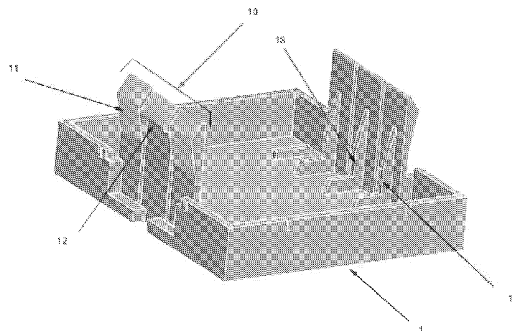
Fig 2 - Center Plate with the snap assembly
