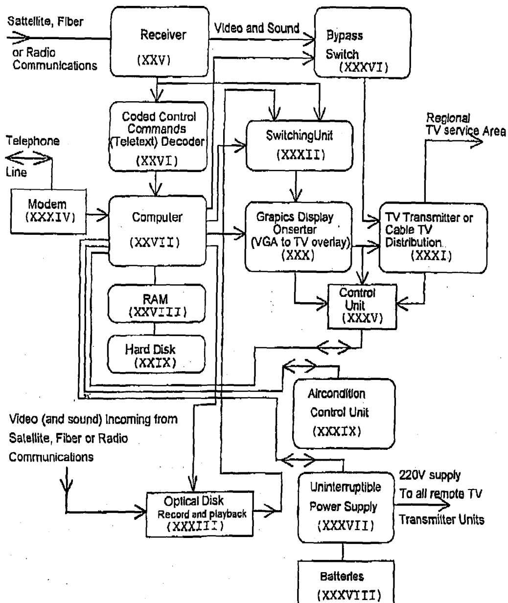
Figure 6 Main Components of a Remote TV Station
