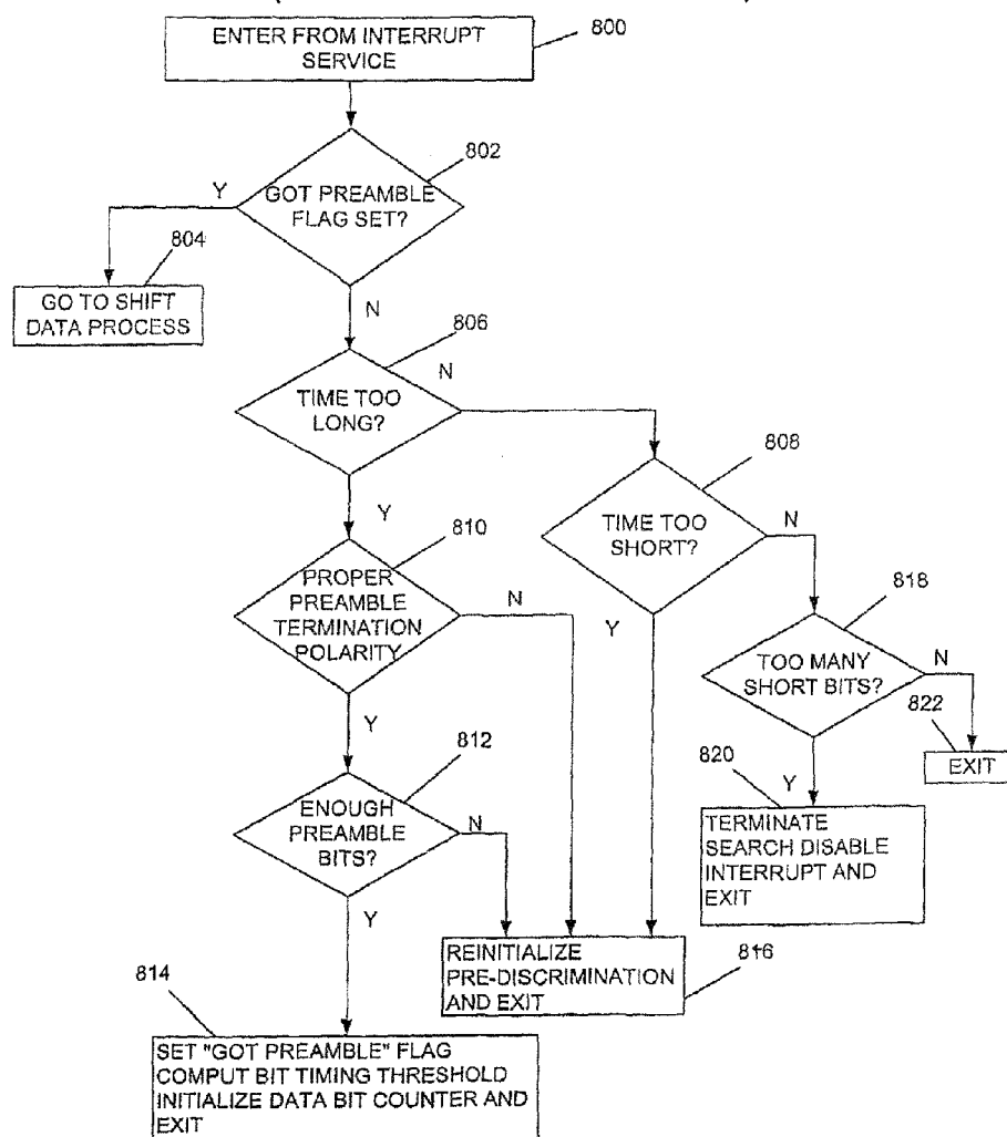
Fig. 45B PACKET PROCESSING (PRE-DISCRIMINATION)
