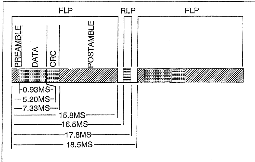
TIMING DIAGRAM WITH PREAMBLE, CRC, POSTAMBLE
