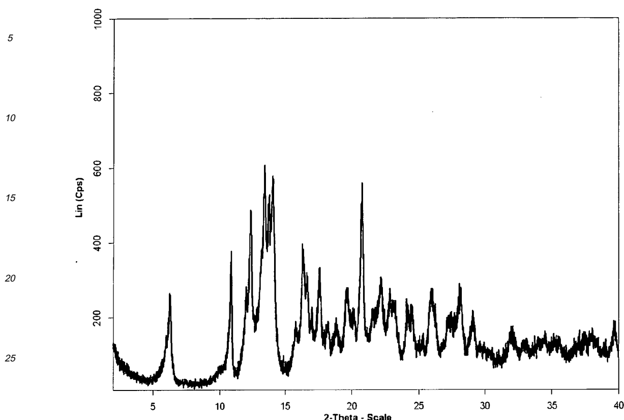
Figure I : Powder diffractogram of 14-O-[(N-3-methyl-2-(R)-amino-butryl-piperidine-3(S)-yl)sulfanyl]acetyl] mutilin hydrochloride
