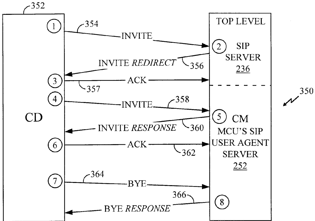
SIP CALL SIGNALING FIG. 11
