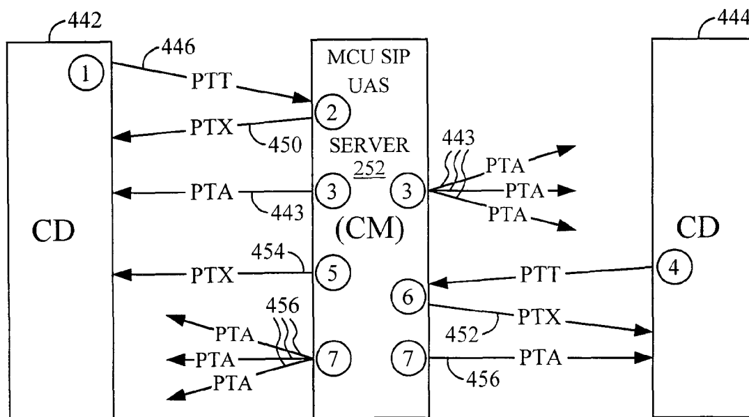
MEDIA SIGNALING MESSAGE SEQUENCE (PRIORITY ARBITRATION)
