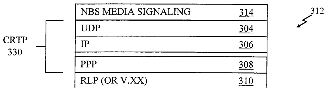
MEDIA SIGNALING PROTOCOL STACK
