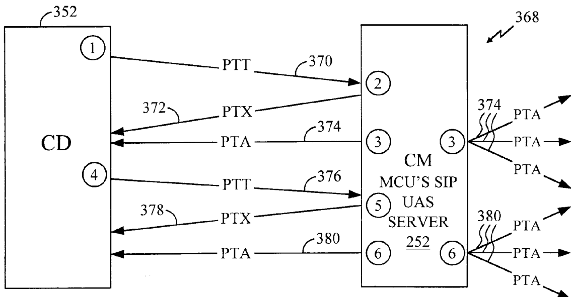
MEDIA SIGNALING MESSAGE SEQUENCE (PTT) FIG. 12
