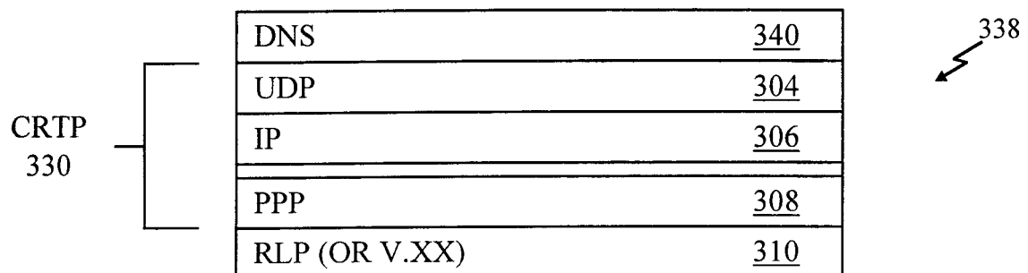
DNS CLIENT PROTOCOL STACK
