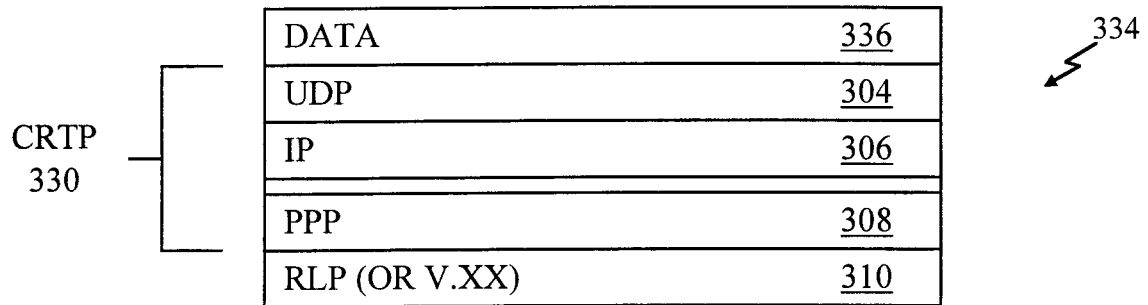
MEDIA TRAFFIC (DATA) PROTOCOL STACK
