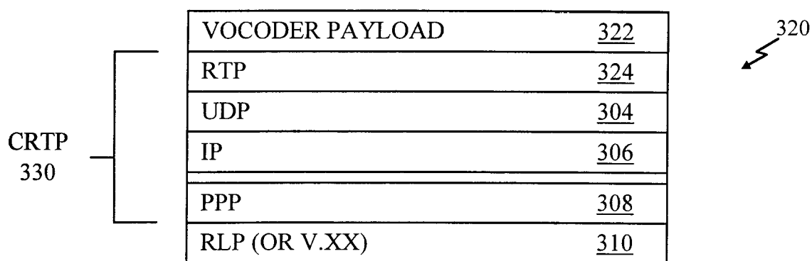
RTP VOICE MEDIA PROTOCOL STACK
