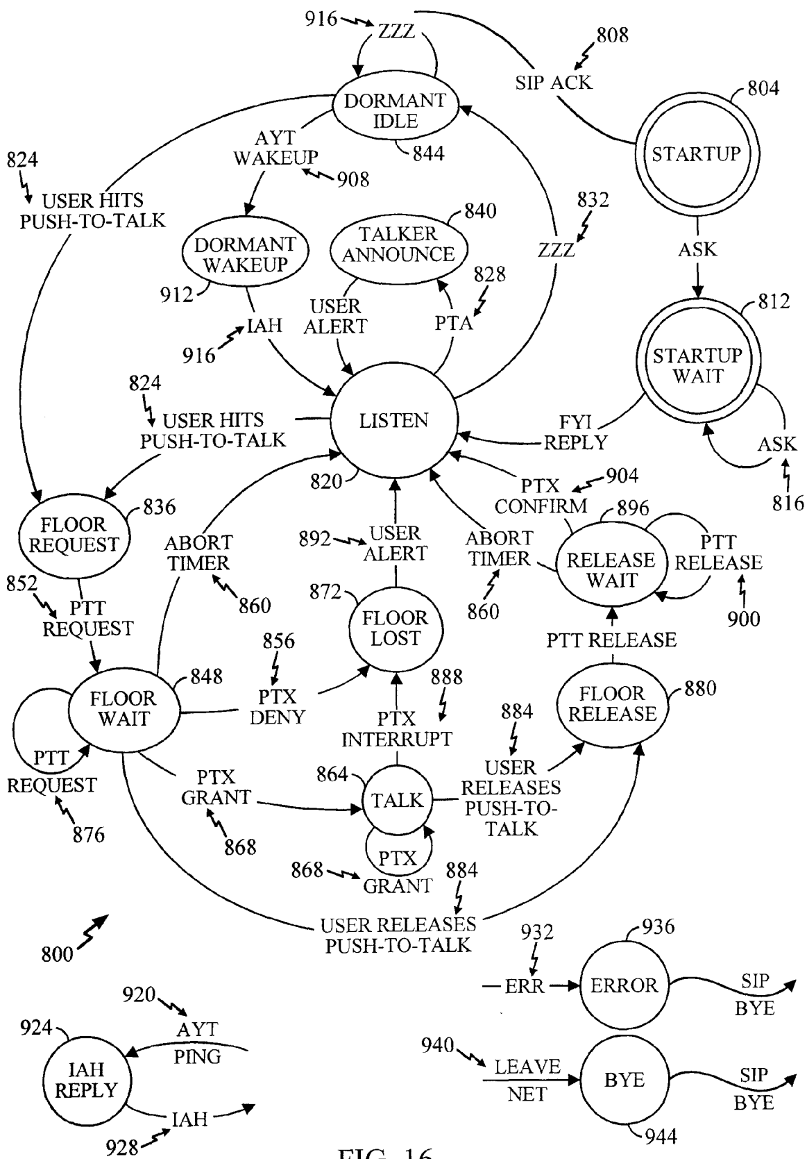
FIG. 16 CD STATE DIAGRAM
