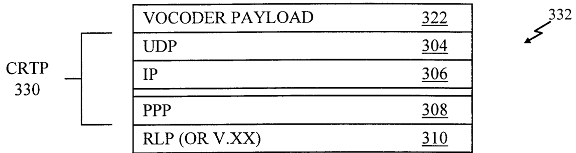
UDP VOICE MEDIA PROTOCOL STACK
