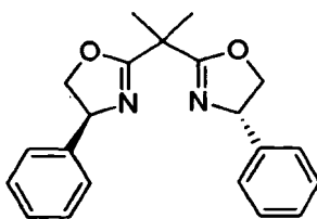
(S,S)-Ph-box
