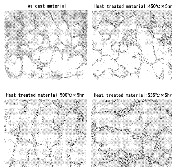
Figure 1 State of crystallized products in AC4CH as-cast material and heat-treated material
