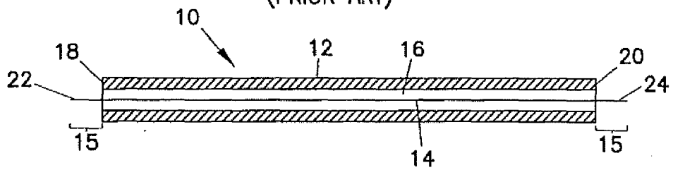
FIG. 2 (PRIOR ART)
