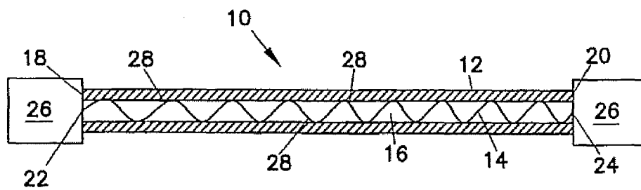
FIG. 3 (PRIOR ART)
