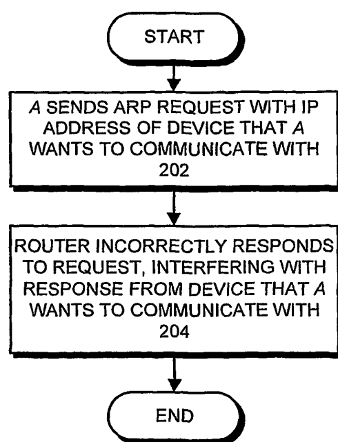
FIG. 2 (PRIOR ART)
