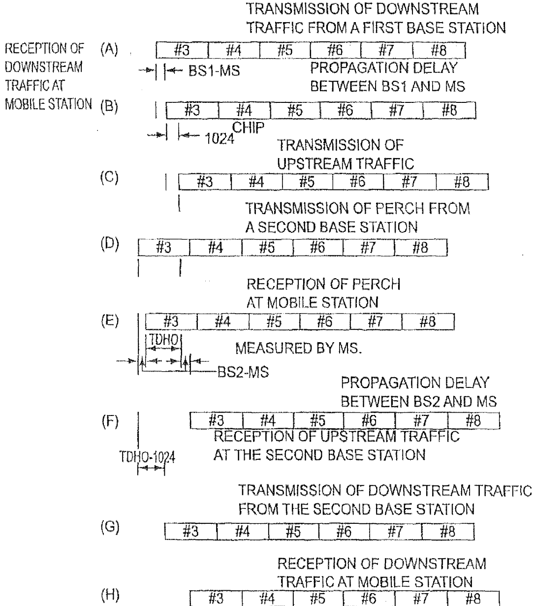
FIG. 16 (PRIOR ART)
