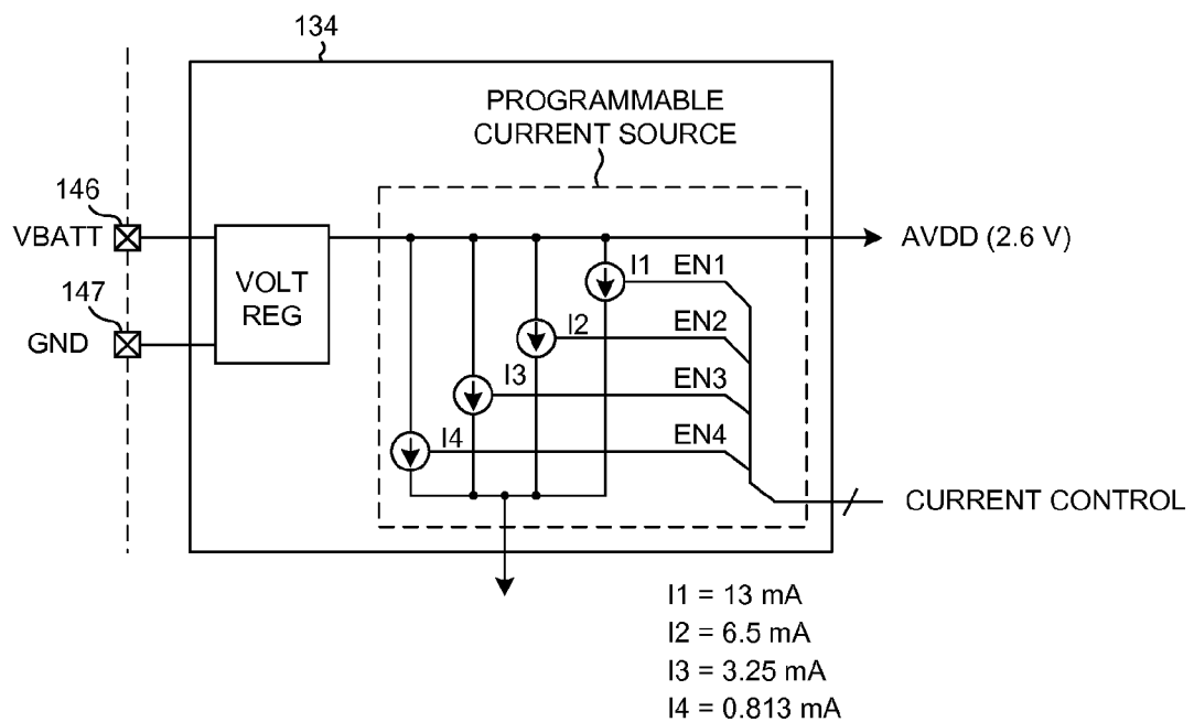
PROGRAMMABLE CURRENT EMBODIMENT
