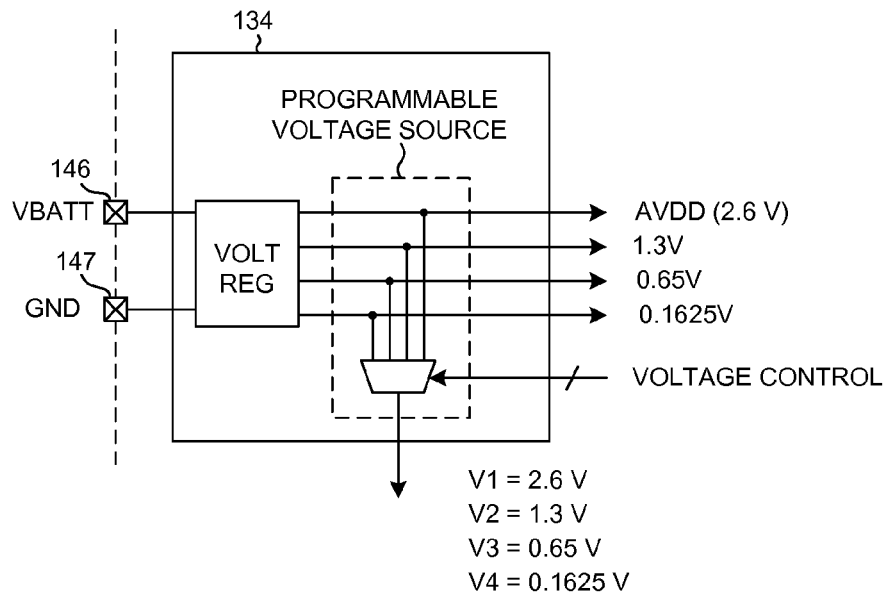
PROGRAMMABLE VOLTAGE EMBODIMENT
