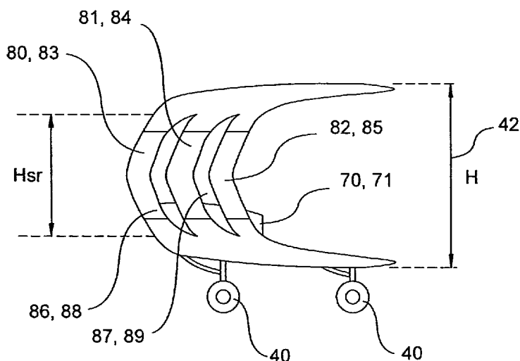
Elevation View Figure 7b
