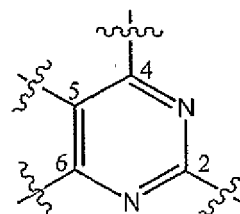
2,4,5,6-substituted pyrimidine
