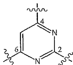
2,4,6-substituted pyrimidine
