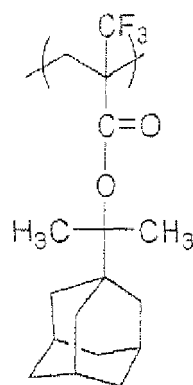
(B-8'')
