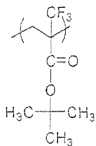
(B-1')
