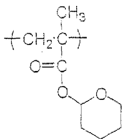
(B-2)
