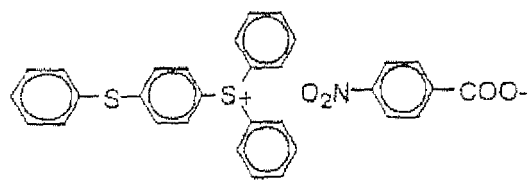
(II-26)
