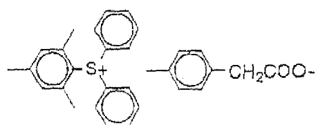
(II-27)
