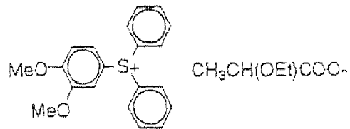
(II-30)
