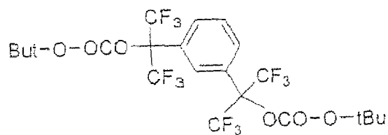
(X-2)
