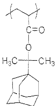
(B-8')
