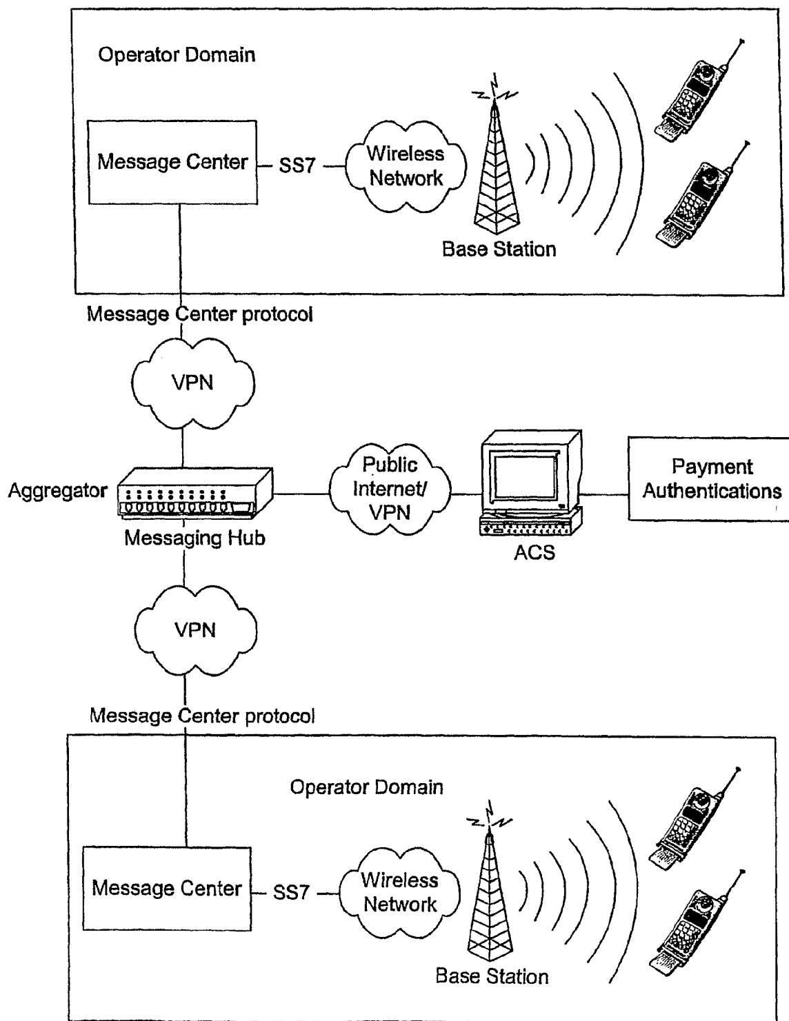
FIG. 15 Two-Way Messaging System
