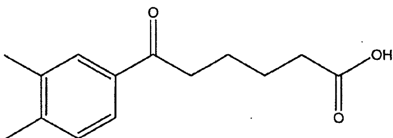
Compound 128
