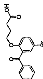
4-(2-Benzoyl-4-chlorophenoxy)butyric acid
