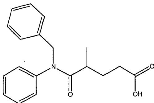
(Compound 12)
