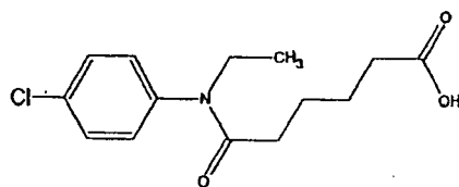
Compound 59
