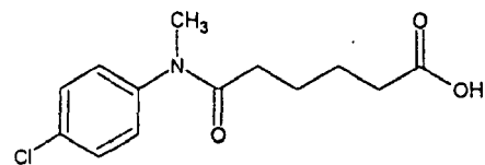
Compound 74
