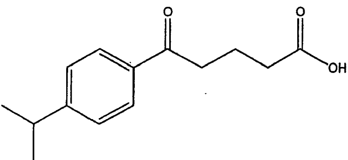
Compound 121
