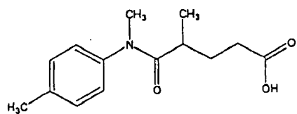
Compound 105
