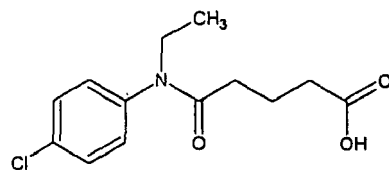
Compound 73
