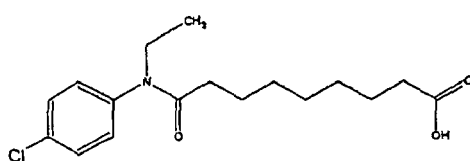
Compound 96
