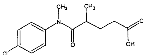
Compound 109
