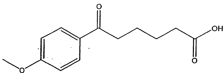
Compound 125
