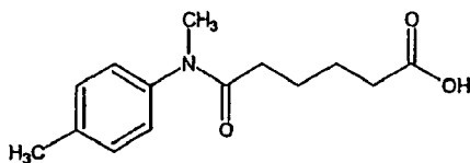
Compound 68
