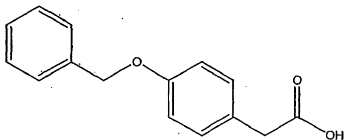
Compound 158 (4-Benzyloxy-phenyl)-acetic acid
