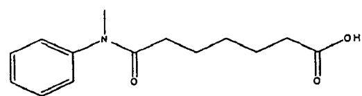
Compound 27
