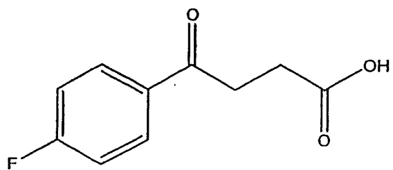
Compound 124
