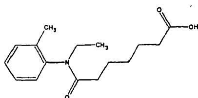
Compound 56
