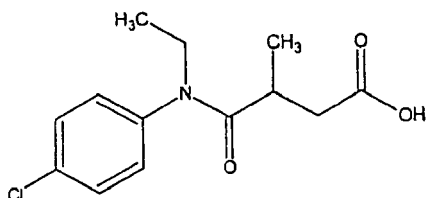
Compound 108
