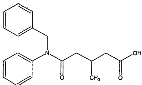
(Compound 10)
