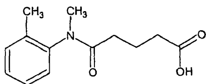
Compound 64
