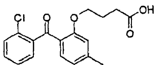
4-(2-(2-Chlorobenzoyl)-5-methylphenoxy)butyric acid
