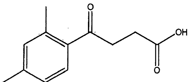
Compound 119
