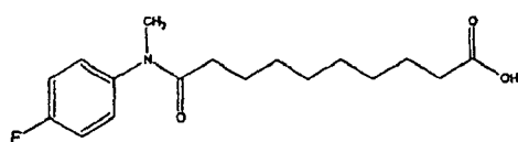
Compound 95
