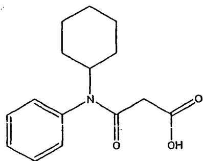
(Compound 3)
