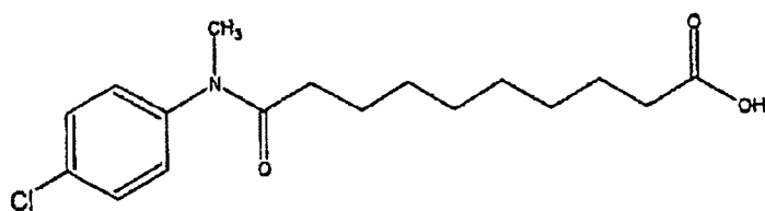
Compound 97
