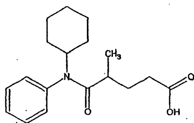
(Compound 14)
