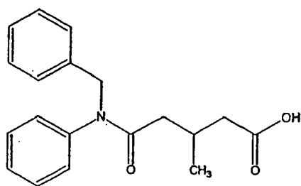
(Compound 10)
