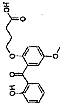
4-(2-(2-Hydroxybenzoyl)-5-methoxyphenoxy)butyric acid
