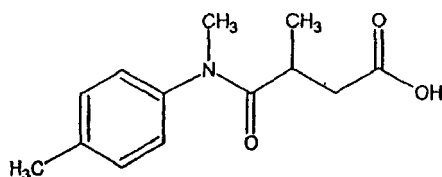
Compound 99
