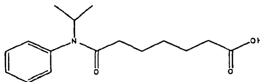
Compound 23
