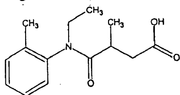
Compound 104
