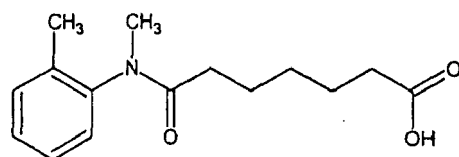
Compound 72
