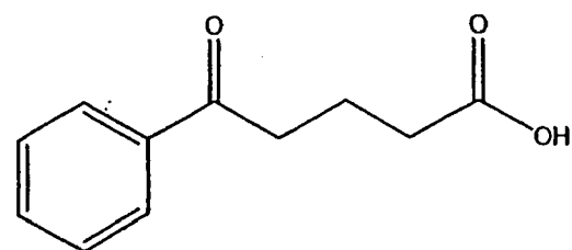
Compound 118
