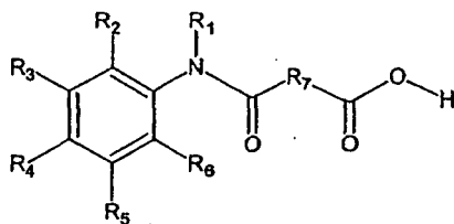
(Compound B)
