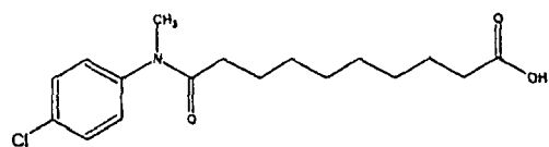
Compound 97
