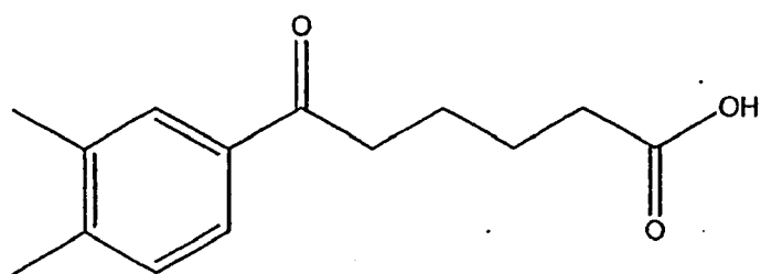
Compound 128
