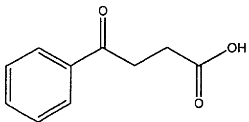
Compound 122
