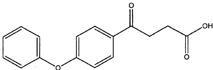
Compound 130
