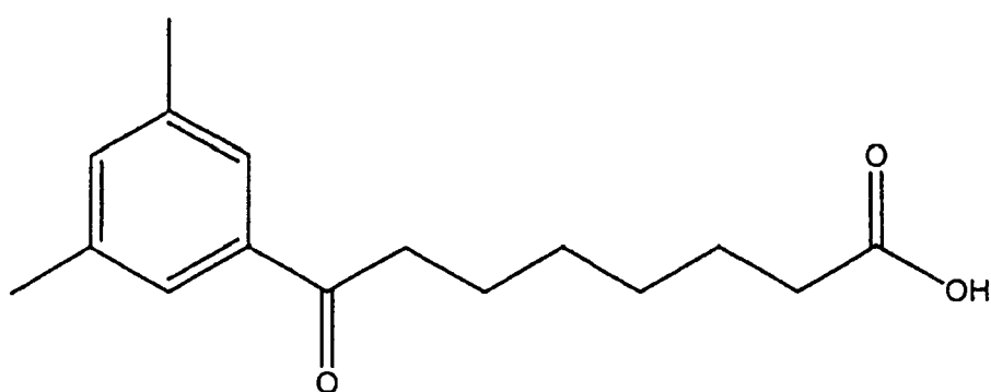
Compound 133
