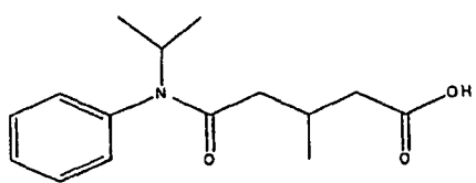
Compound 25
