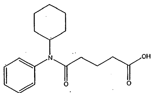
(Compound 6)
