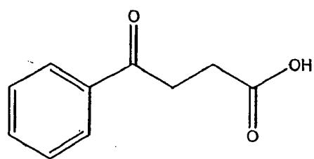
Compound 122
