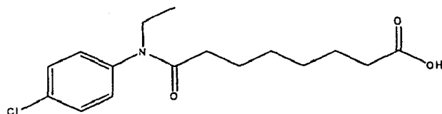
Compound 33
