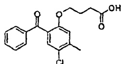
4-(2-Benzoyl-4-chloro-3-methylphenoxy)butyric acid
