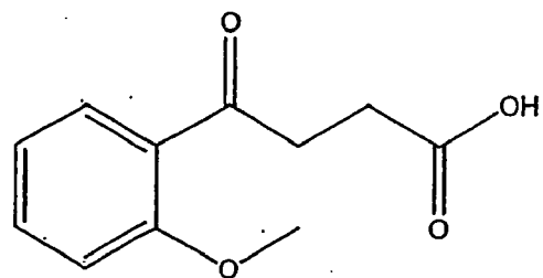
Compound 123
