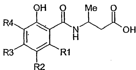
(Compound D)
