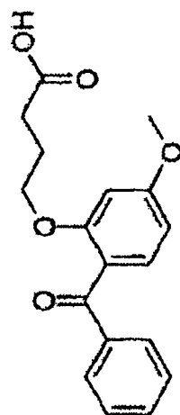
4-(2-Benzoyl-5-methoxyphenoxy)butyric
