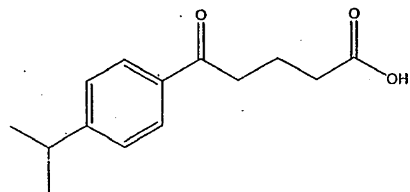
Compound 121
