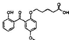
Sodium 8-(2-(2-Hydroxybenzoyl)phenoxy)octanoate
