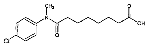
Compound 83
