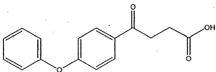
Compound 130
