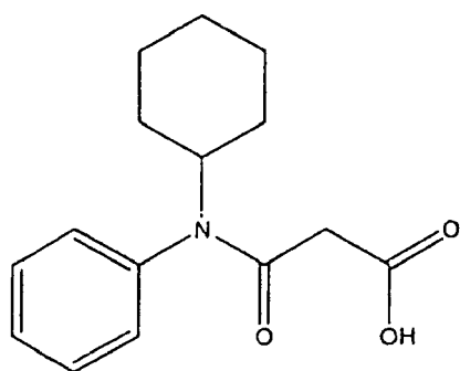
(Compound 3)
