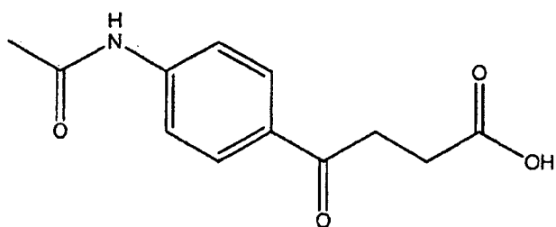
Compound 112
