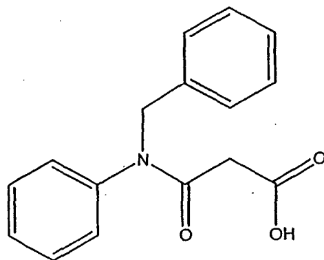
(Compound 1)
