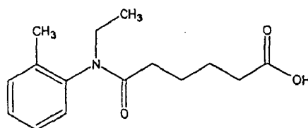
Compound 43
