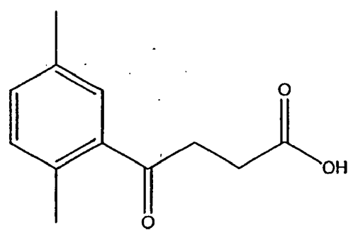
Compound 132
