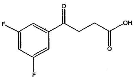
Compound 117
