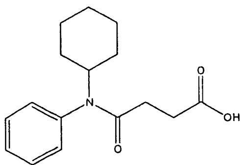
(Compound 4)
