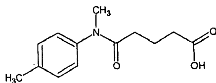
Compound 63
