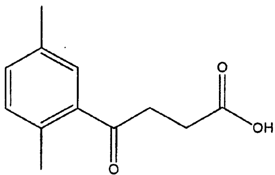
Compound 132
