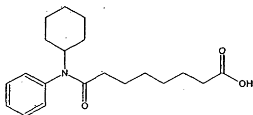
(Compound 18)
