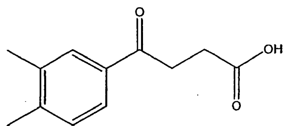
Compound 129
