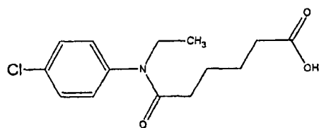
Compound 59
