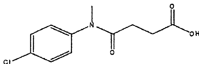
Compound 29
