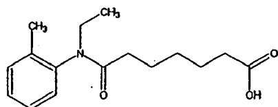
Compound 42
