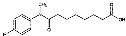
Compound 79
