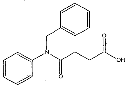
(Compound 2)
