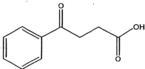
Compound 111
