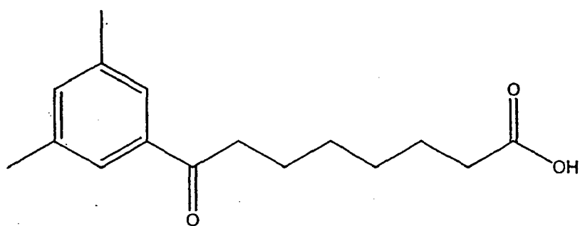
Compound 133
