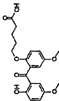
5-(2-(2-Hydroxy-5-methoxybenzoyl)-4-methoxyphenoxy) valeric acid
