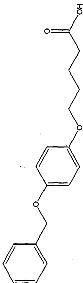
Compound 178 5-(4-Benzoyloxy-phenoxy)-pentanoic add
