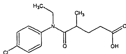
Compound 38
