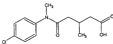
Compound 107
