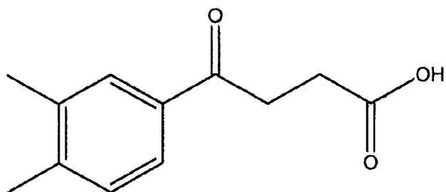
Compound 129
