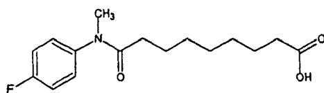
Compound 81
