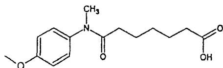
Compound 77
