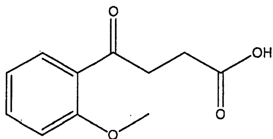
Compound 123
