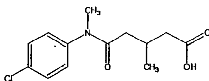
Compound 107
