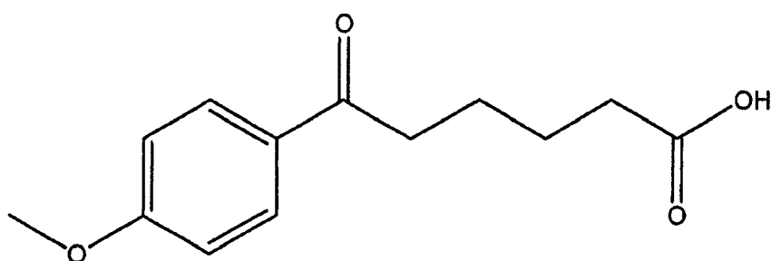
Compound 125
