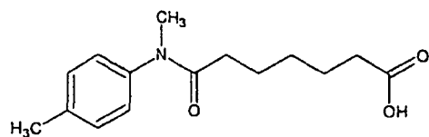
Compound 71
