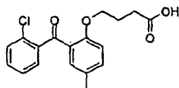
4-(2-(2-Chlorobenzoyl)-4-methylphenoxy)butyric acid
