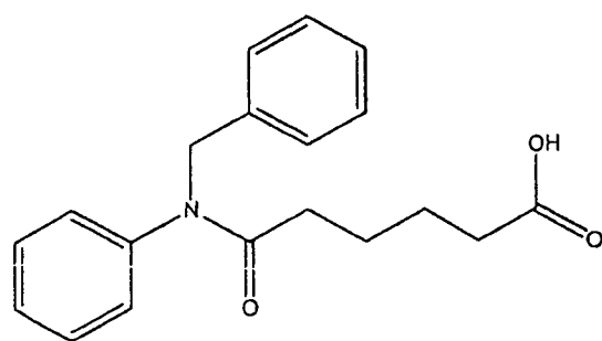
(Compound 7)
