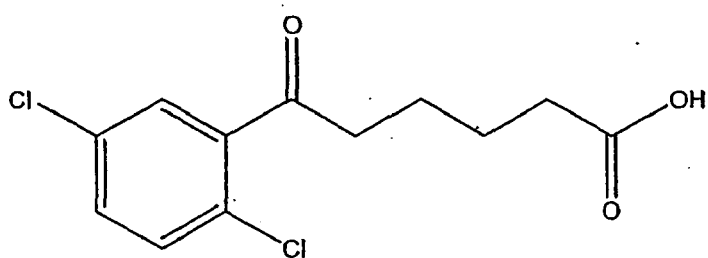
Compound 134
