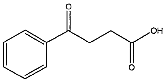
Compound 111
