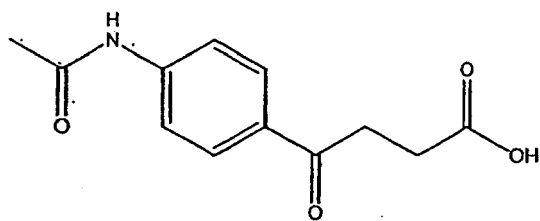
Compound 112
