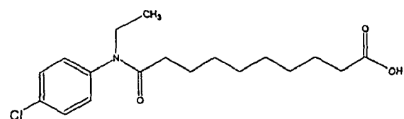
Compound 98
