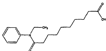
Compound 58
