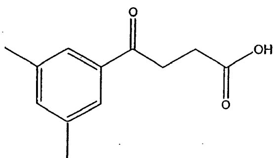
Compound 126
