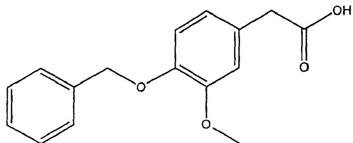
Compound 155 (4-Benzyloxy-3-methoxyphenyl)-acetic acid
