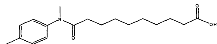
Compound 35
