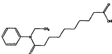
Compound 58
