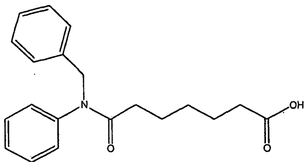
(Compound 17)
