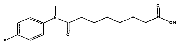
Compound 34
