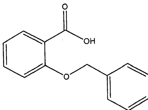
Compound 159
