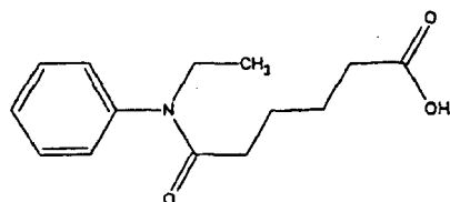
Compound 55
