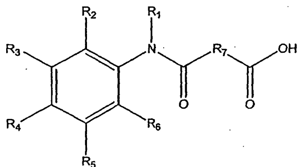
Compound A
