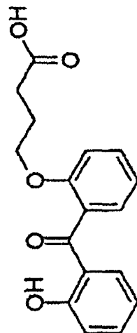
4-(2-(2-Hydroxybenzoyl)phenoxy)butyric
