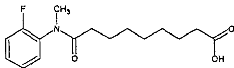
Compound 80
