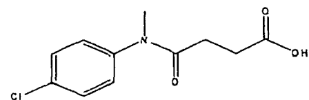
Compound 29
