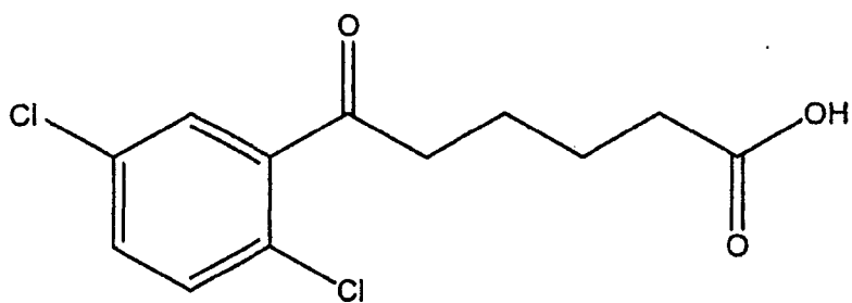
Compound 134
