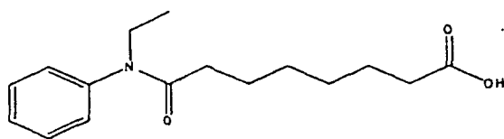
Compound 32
