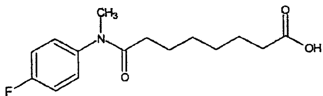
Compound 79
