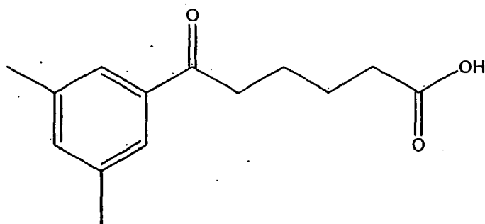
Compound 138
