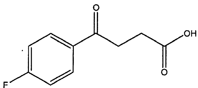
Compound 124
