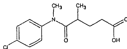
Compound 45
