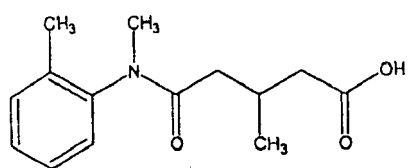
Compound 103
