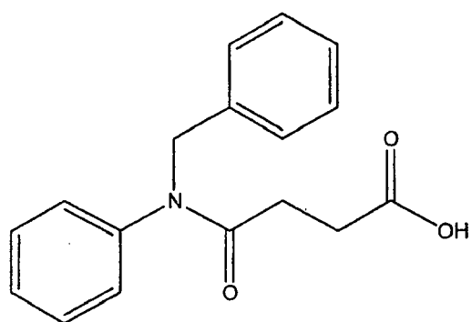
(Compound 2)
