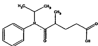
Compound 48
