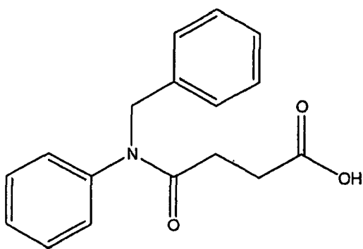
(Compound 2)
