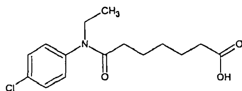
Compound 82
