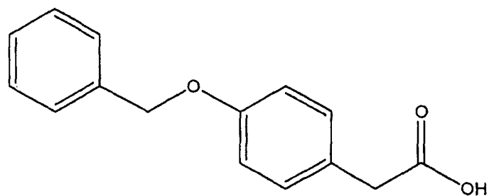
Compound 158 (4-Benzyloxy-phenyl)-acetic acid
