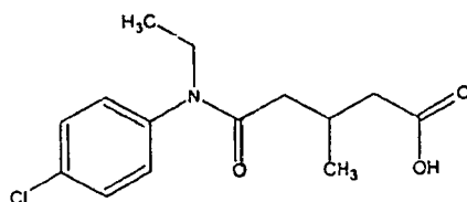
Compound 110
