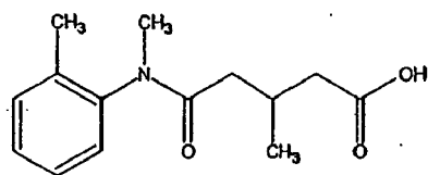
Compound 103
