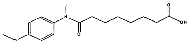
Compound 31
