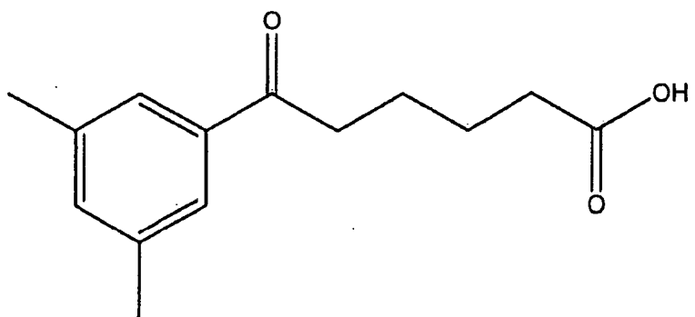
Compound 138
