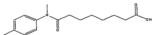
Compound 30
