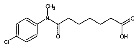
Compound 75
