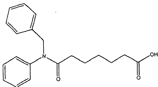
(Compound 17)
