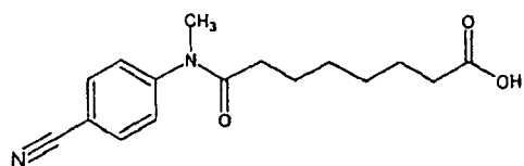
Compound 78
