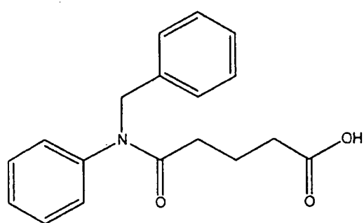
(Compound 5)
