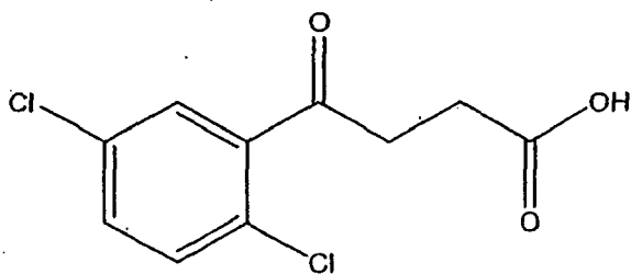
Compound 136
