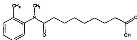
Compound 54
