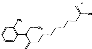
Compound 57
