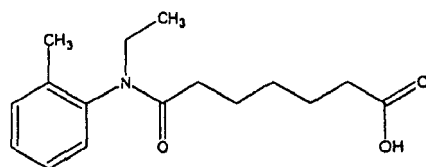
Compound 42
