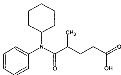
(Compound 14)
