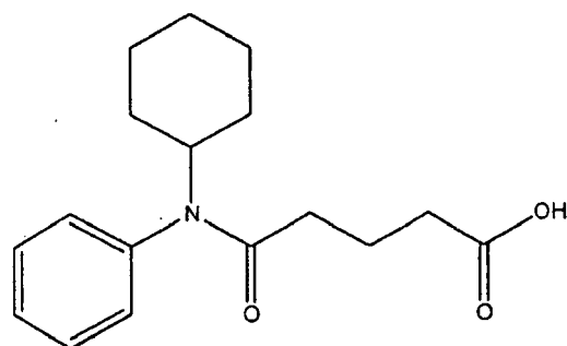
(Compound 6)
