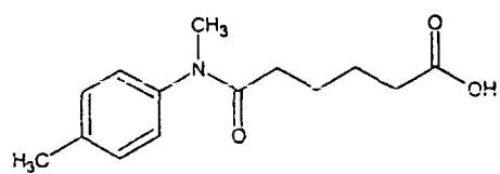
Compound 68
