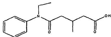
Compound 26
