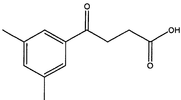
Compound 126
