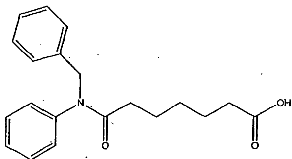
(Compound 17)
