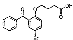
4-(2-Benzoyl-4-bromophenoxy)butyric acid
