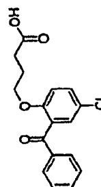
4-(2-Benzoyl-4-chlorophenoxy)butyric acid
