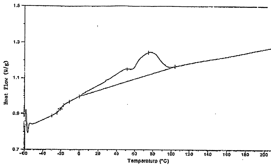
Figure 4 DSC Plot of Sample 20
