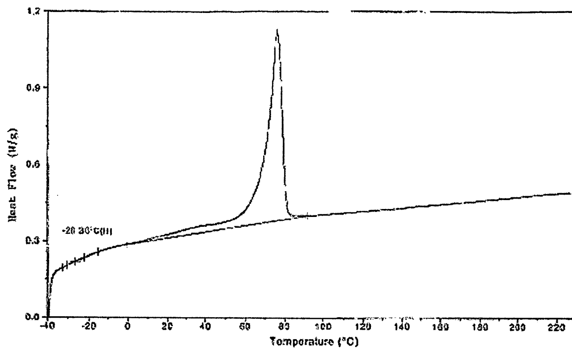
Figure 3 DSC Plot of Sample 29
