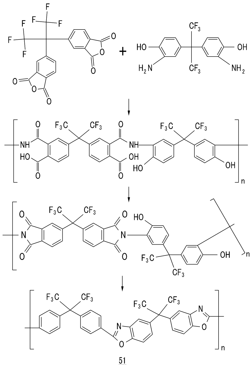
[Reaction Scheme 3]
