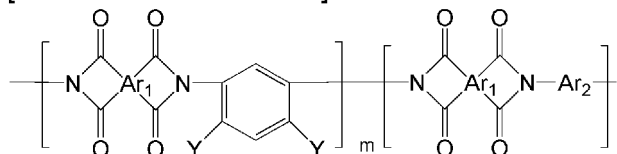
[Chemical Formula 39]
