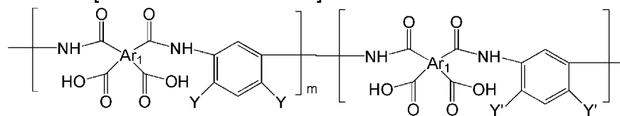
[Chemical Formula 12]
