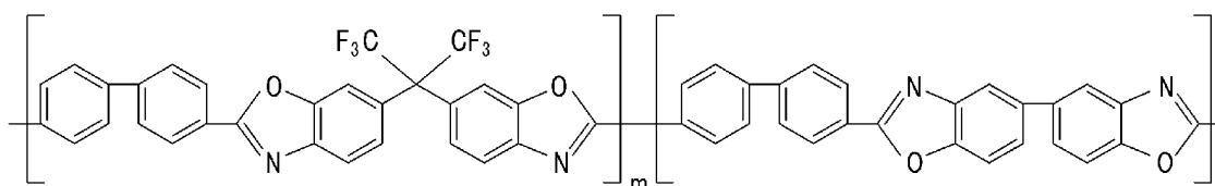
[Chemical Formula 56]
