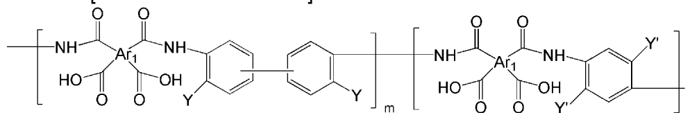
[Chemical Formula 16]
