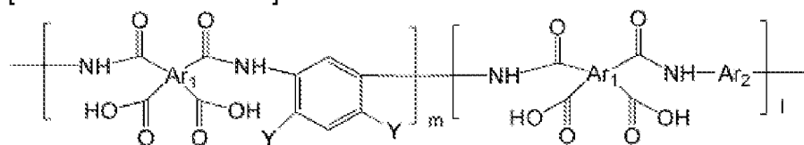
[Chemical Formula 7]
