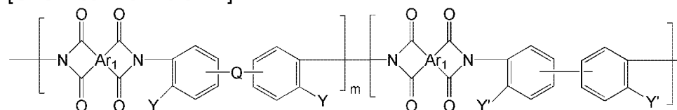
[Chemical Formula 41]
