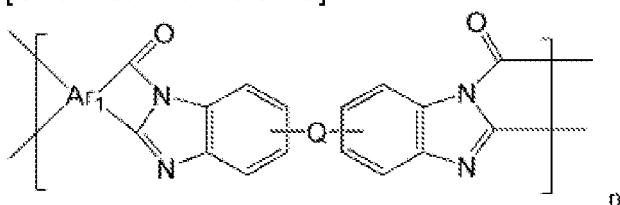
[Chemical Formula 20]
