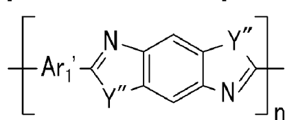
[Chemical Formula 24]
