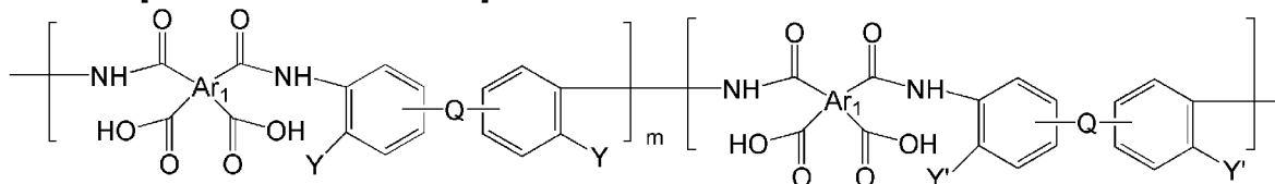
[Chemical Formula 10]
