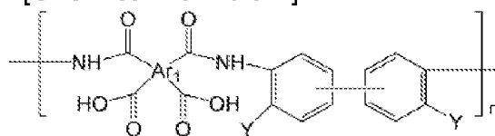
[Chemical Formula 2]
