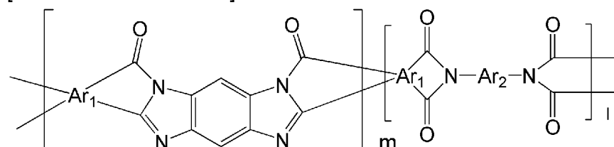
[Chemical Formula 32]
