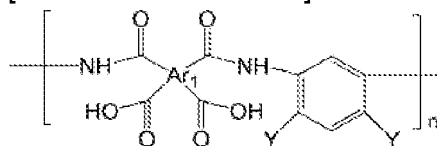
[Chemical Formula 3]
