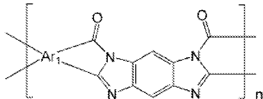
[Chemical Formula 25]
