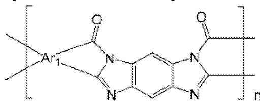
[Chemical Formula 25]
