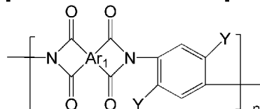
[Chemical Formula 36]
