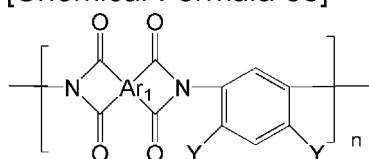
[Chemical Formula 35]
