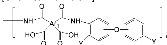
[Chemical Formula 1]
