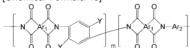
[Chemical Formula 40]
