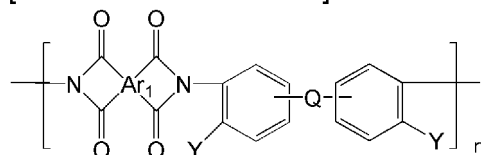
[Chemical Formula 33]
