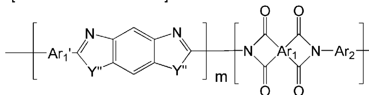
[Chemical Formula 30]
