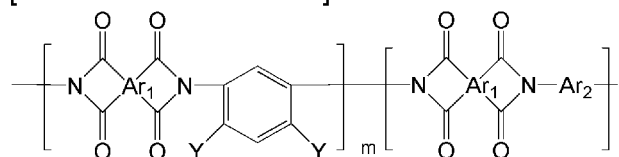
[Chemical Formula 39]
