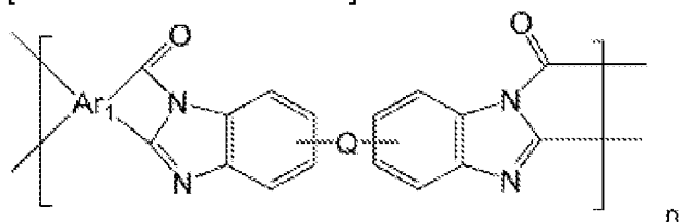
[Chemical Formula 20]
