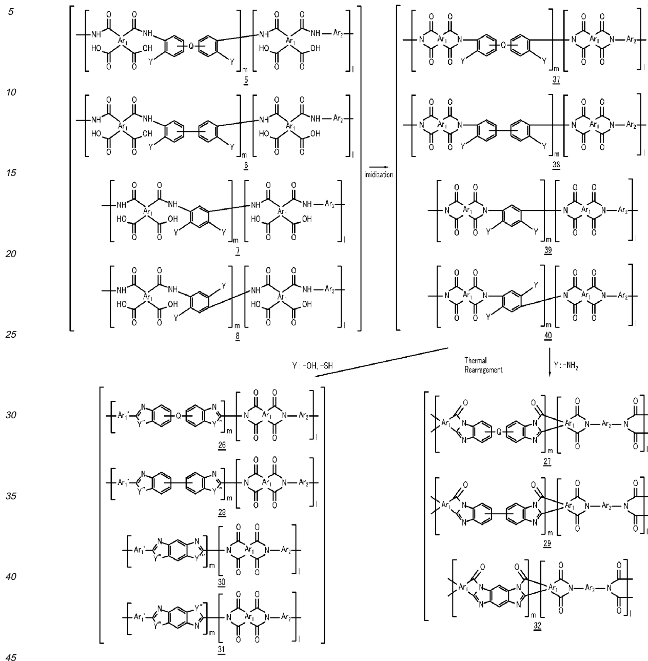
[Reaction Scheme 2]
