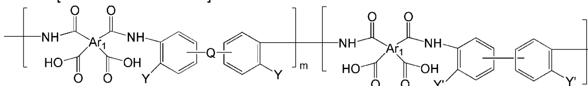
[Chemical Formula 9]
