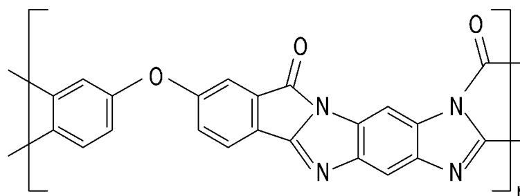
[Chemical Formula 55]
