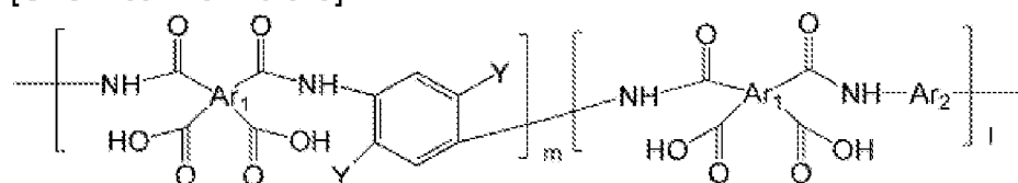
[Chemical Formula 8]
