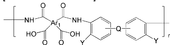
[Chemical Formula 1]
