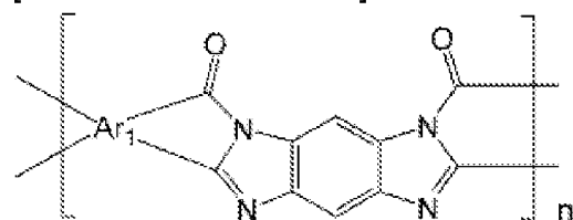
[Chemical Formula 25]
