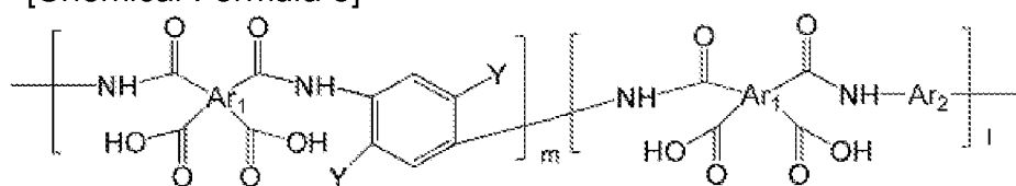
[Chemical Formula 8]
