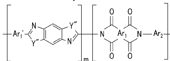
[Chemical Formula 31]
