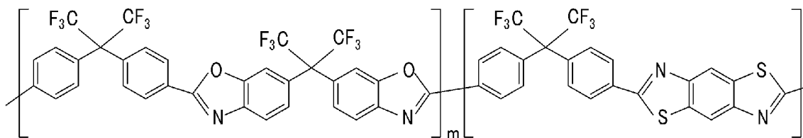
[Chemical Formula 62]
