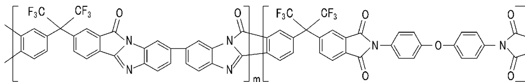
[Chemical Formula 58]
