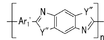
[Chemical Formula 24]
