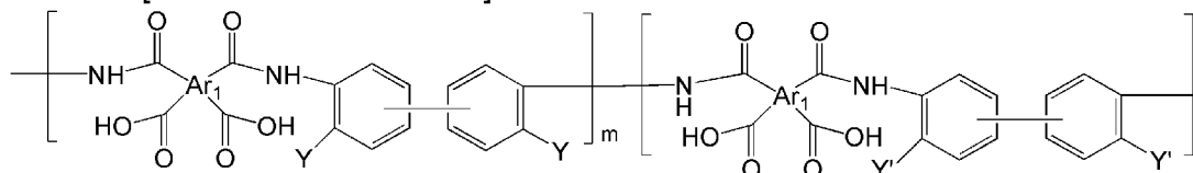
[Chemical Formula 11]
