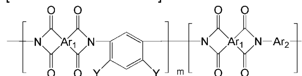
[Chemical Formula 39]
