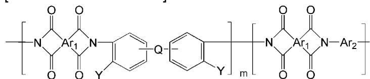
[Chemical Formula 37]
