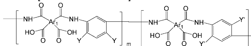
[Chemical Formula 17]
