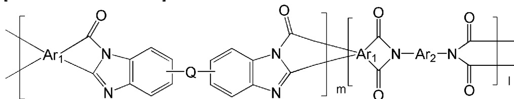
[Chemical Formula 27]
