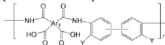
[Chemical Formula 2]
