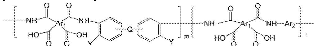
[Chemical Formula 5]
