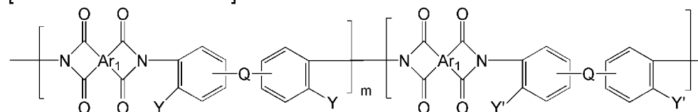
[Chemical Formula 42]
