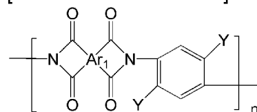
[Chemical Formula 36]
