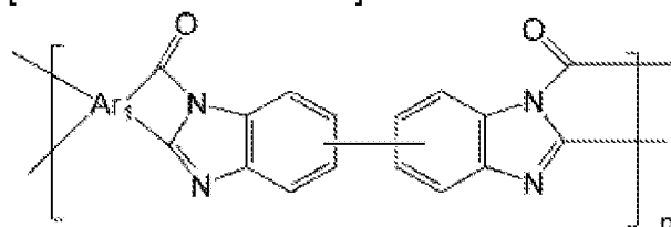
[Chemical Formula 22]
