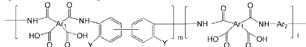
[Chemical Formula 6]
