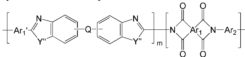
[Chemical Formula 26]
