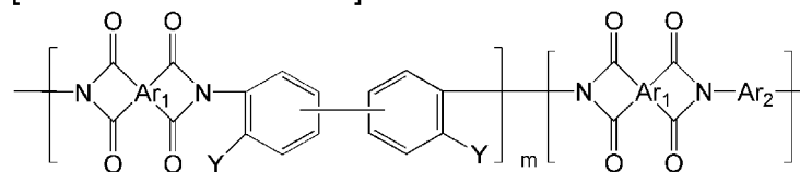
[Chemical Formula 38]
