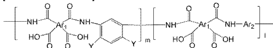
[Chemical Formula 7]
