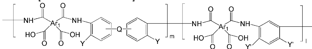
[Chemical Formula 13]
