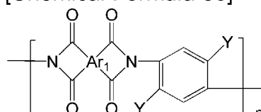
[Chemical Formula 36]
