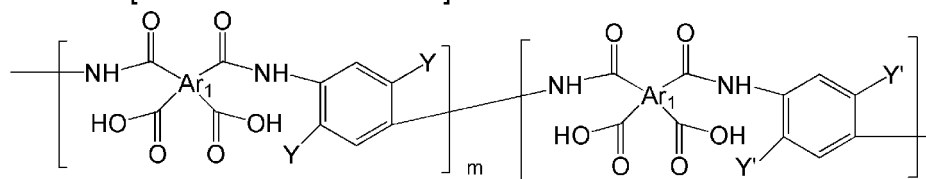
[Chemical Formula 18]
