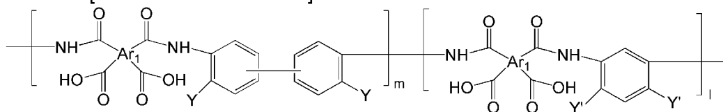
[Chemical Formula 14]
