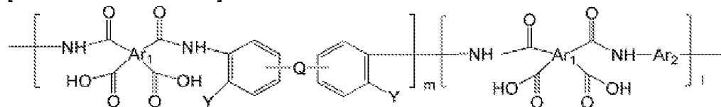
[Chemical Formula 5]
