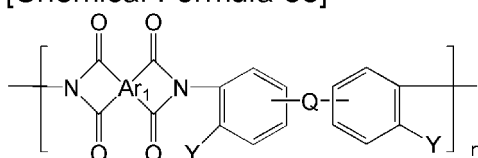
[Chemical Formula 33]
