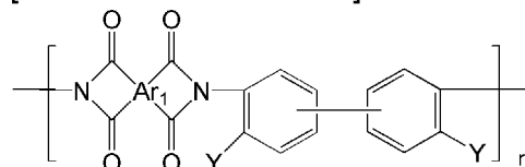
[Chemical Formula 34]
