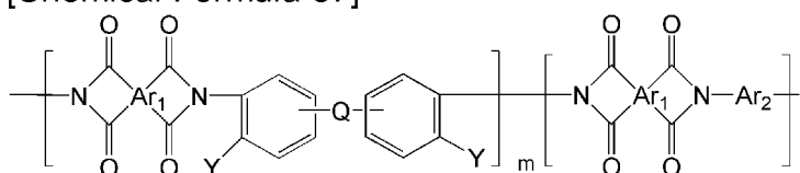
[Chemical Formula 37]
