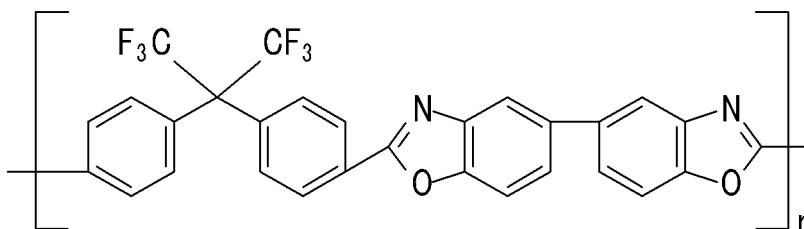
[Chemical Formula 54]
