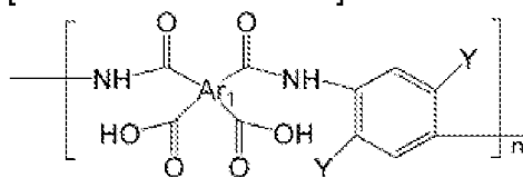
[Chemical Formula 4]
