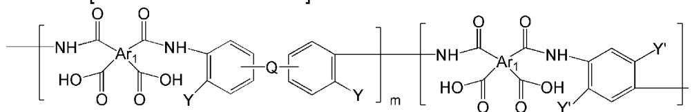
[Chemical Formula 15]
