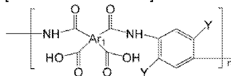
[Chemical Formula 4]
