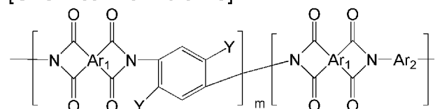
[Chemical Formula 40]
