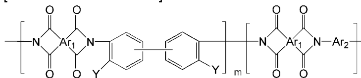
[Chemical Formula 38]
