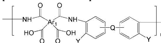
[Chemical Formula 1]
