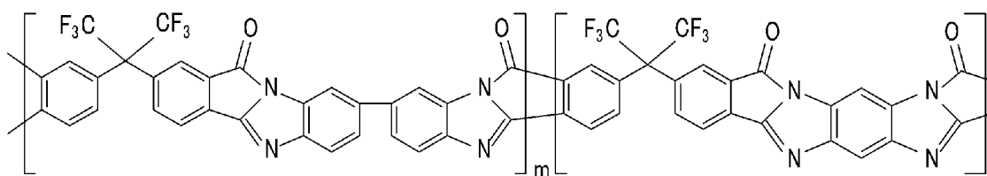
[Chemical Formula 61]
