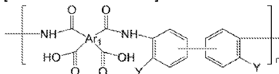
[Chemical Formula 2]
