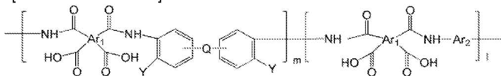
[Chemical Formula 5]
