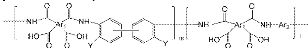
[Chemical Formula 6]
