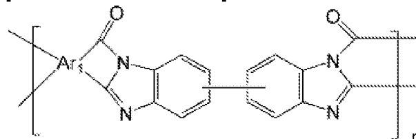
[Chemical Formula 22]
