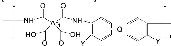
[Chemical Formula 1]
