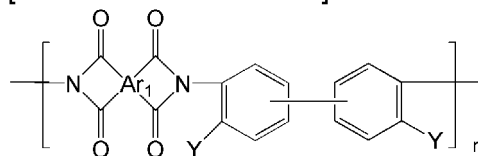
[Chemical Formula 34]
