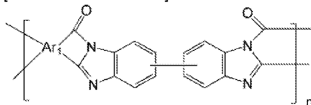
[Chemical Formula 22]
