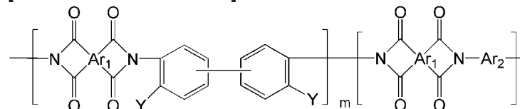
[Chemical Formula 38]
