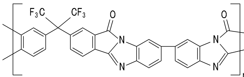
[Chemical Formula 53]
