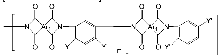
[Chemical Formula 49]
