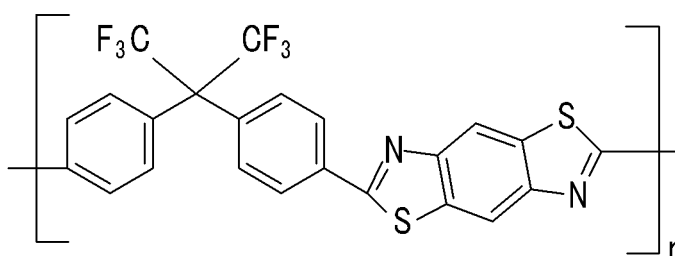
[Chemical Formula 52]
