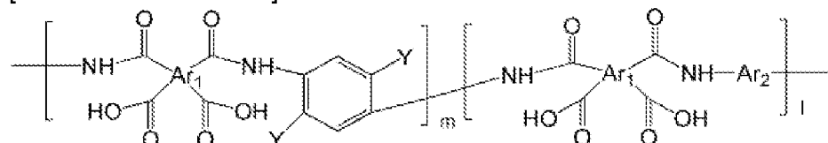
[Chemical Formula 8]
