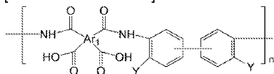
[Chemical Formula 2]
