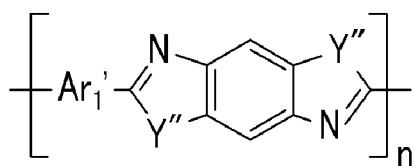
[Chemical Formula 24]
