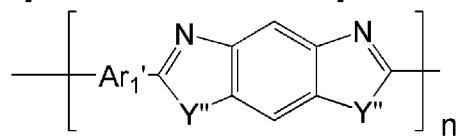
[Chemical Formula 23]
