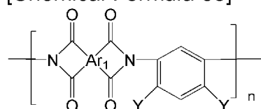
[Chemical Formula 35]
