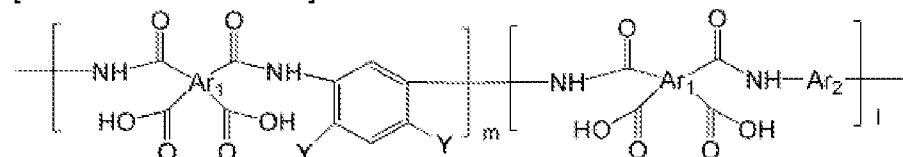
[Chemical Formula 7]
