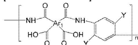
[Chemical Formula 4]
