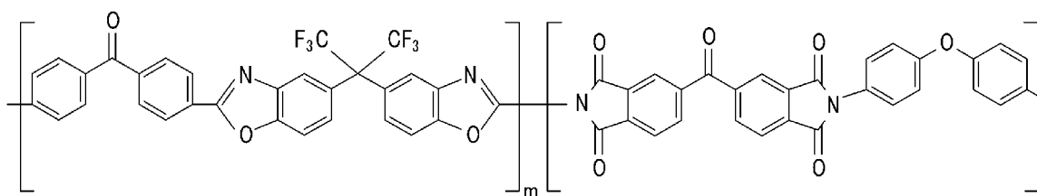
[Chemical Formula 57]
