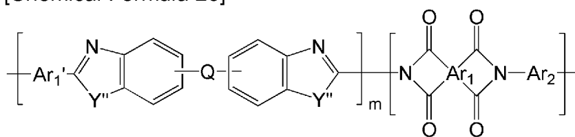
[Chemical Formula 26]
