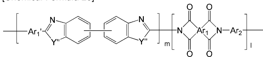
[Chemical Formula 28]
