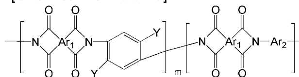
[Chemical Formula 40]
