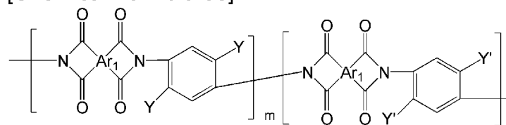
[Chemical Formula 50]
