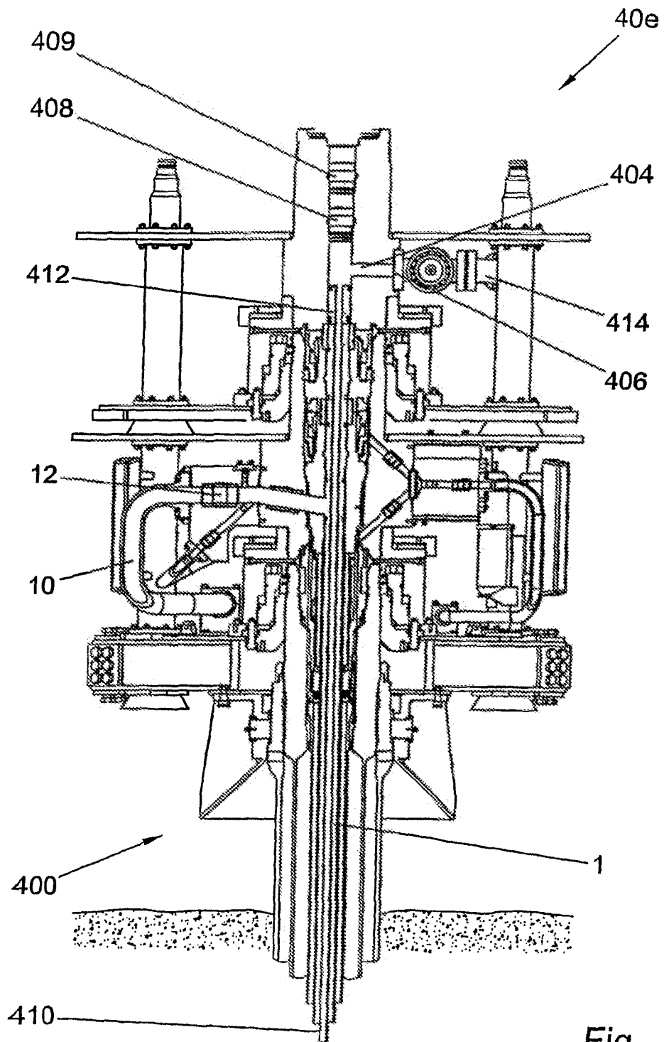
TYPICAL SECTION
