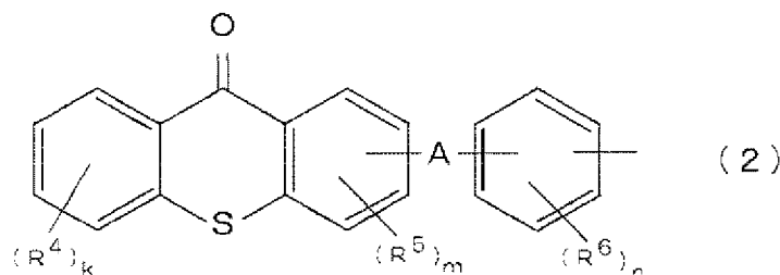
[Chem. 2]
