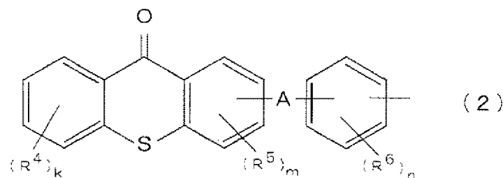
[Chem. 2]
