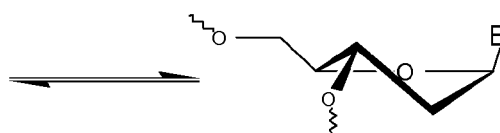
C 3'-endo (N-type)
