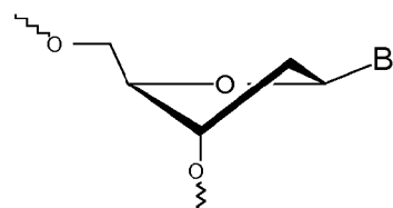
C 2'-endo (S-type)
