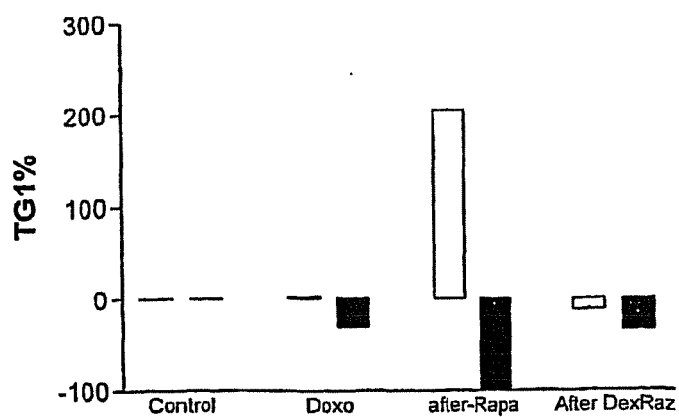
Fig. 3c The effect of doxorubicine on the length of the G1 phase of the cell cycle
