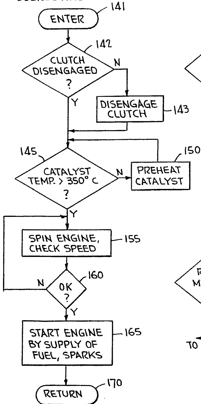
FIG. 9(a) ENGINE STARTING SUBROUTINE
