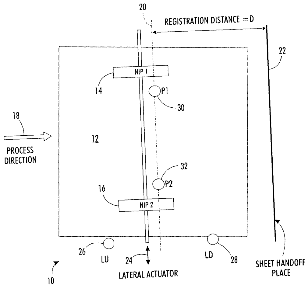
FIG. 1 PRIOR ART
