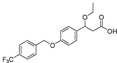
(7A) Ethyl 3-ethoxy-3-(4-((4-(trifluoromethyl)benzyl)oxy)phenyl)propionate
