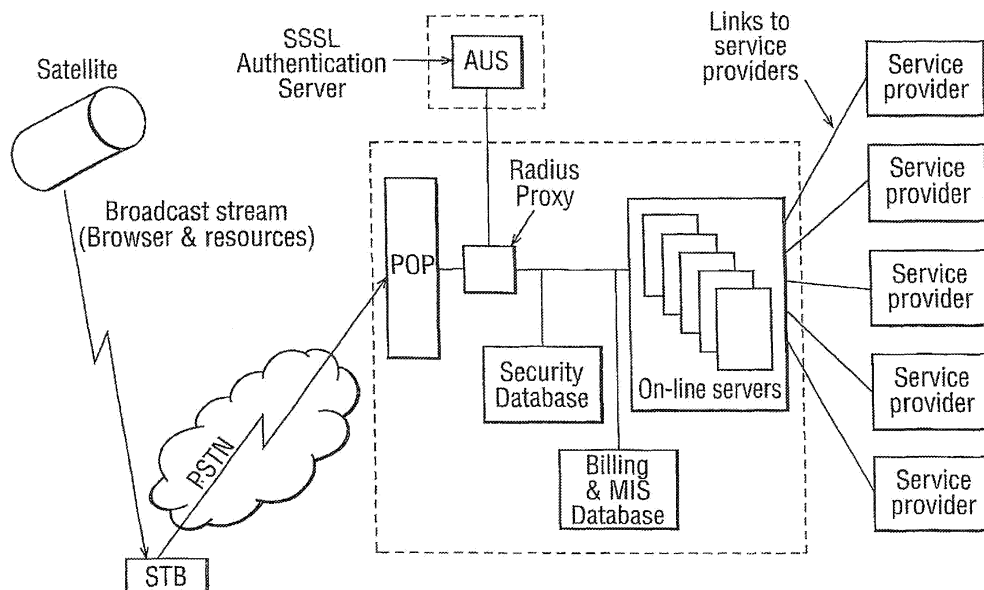
FIG.1 : Overview of WapTV Infrastructure
