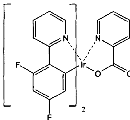
F 2 Irpic
