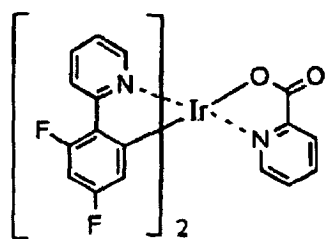
F 2 Irpic
