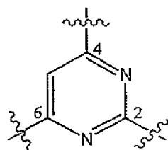
2,4,6-substituted pyrimidine
