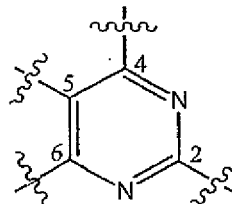
2,4,5,6-substituted pyrimidine
