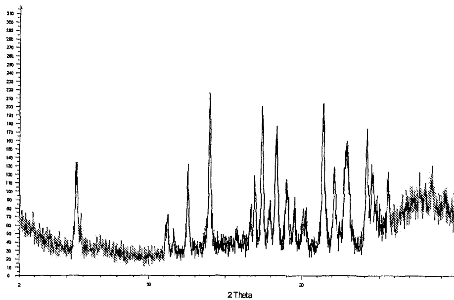
Figure 1.4 Polymorph IV
