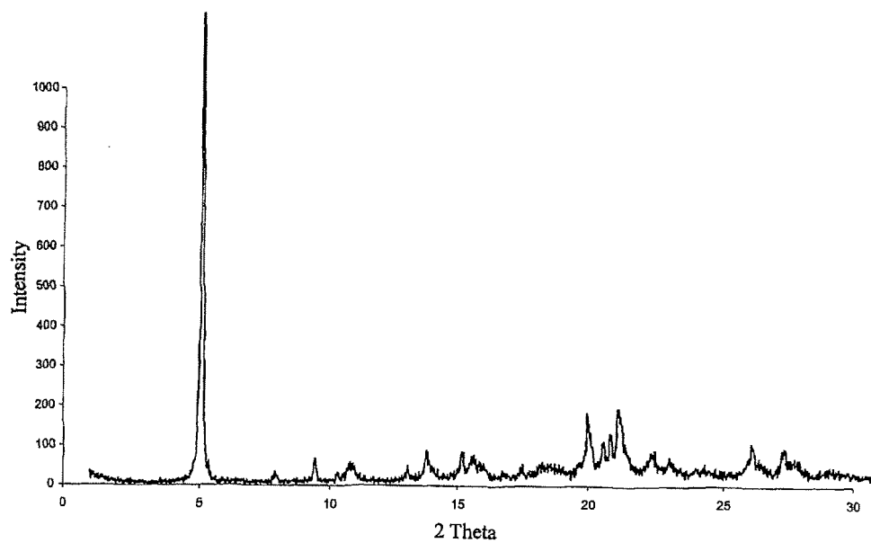
Figure 1.2 Polymorph II
