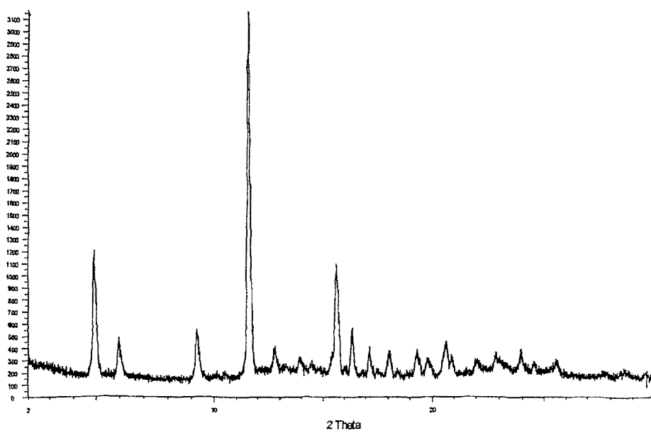
Figure 1.4 Polymorph IV
