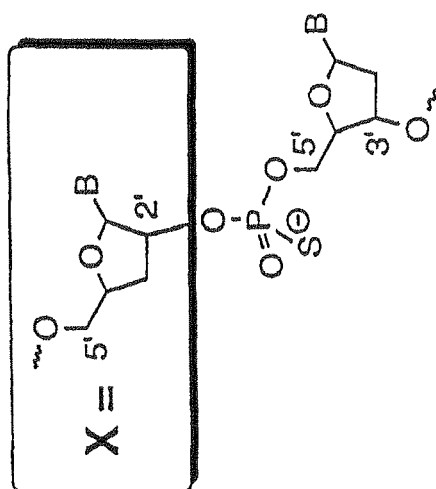
3'-Deoxynucleoside
