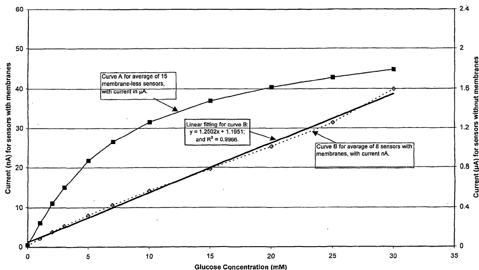
Figure 3. Calibration Curves at 37 °C
