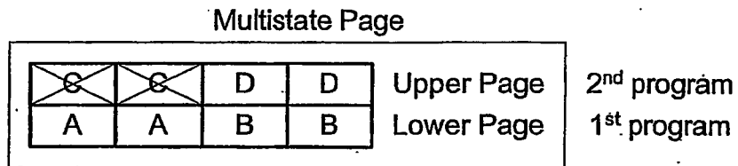
Non-robust Arrangement of Duplicate Sectors in a Page
