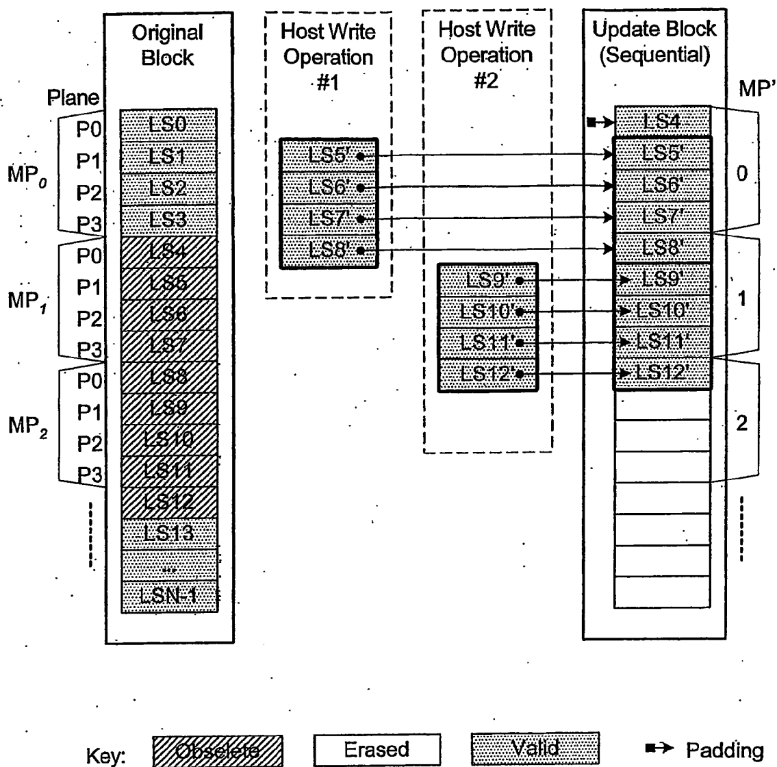
PLANE-ALIGNED SEQUENTIAL UPDATE Example
