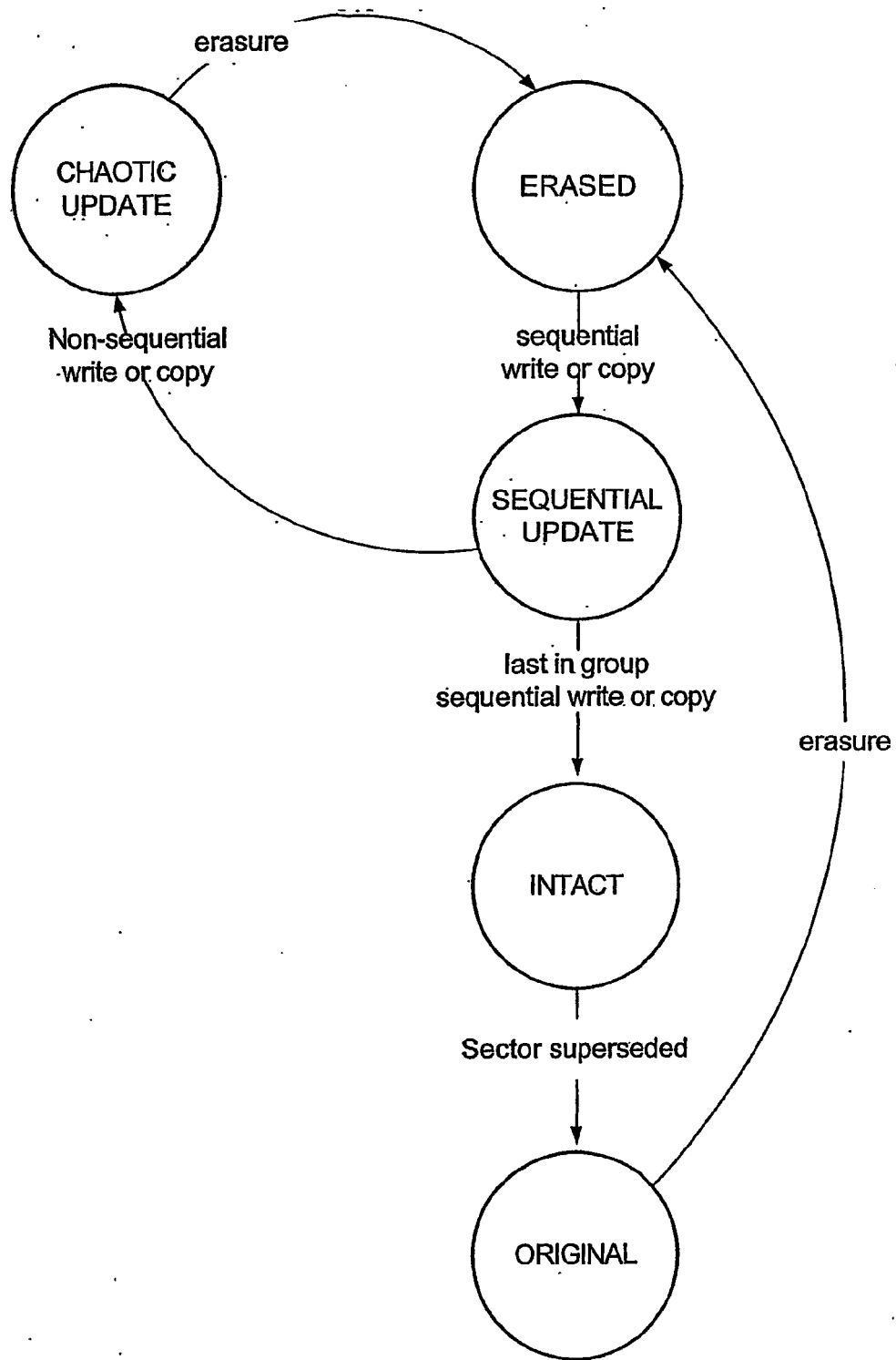
PHYSICAL METABLOCK STATES
