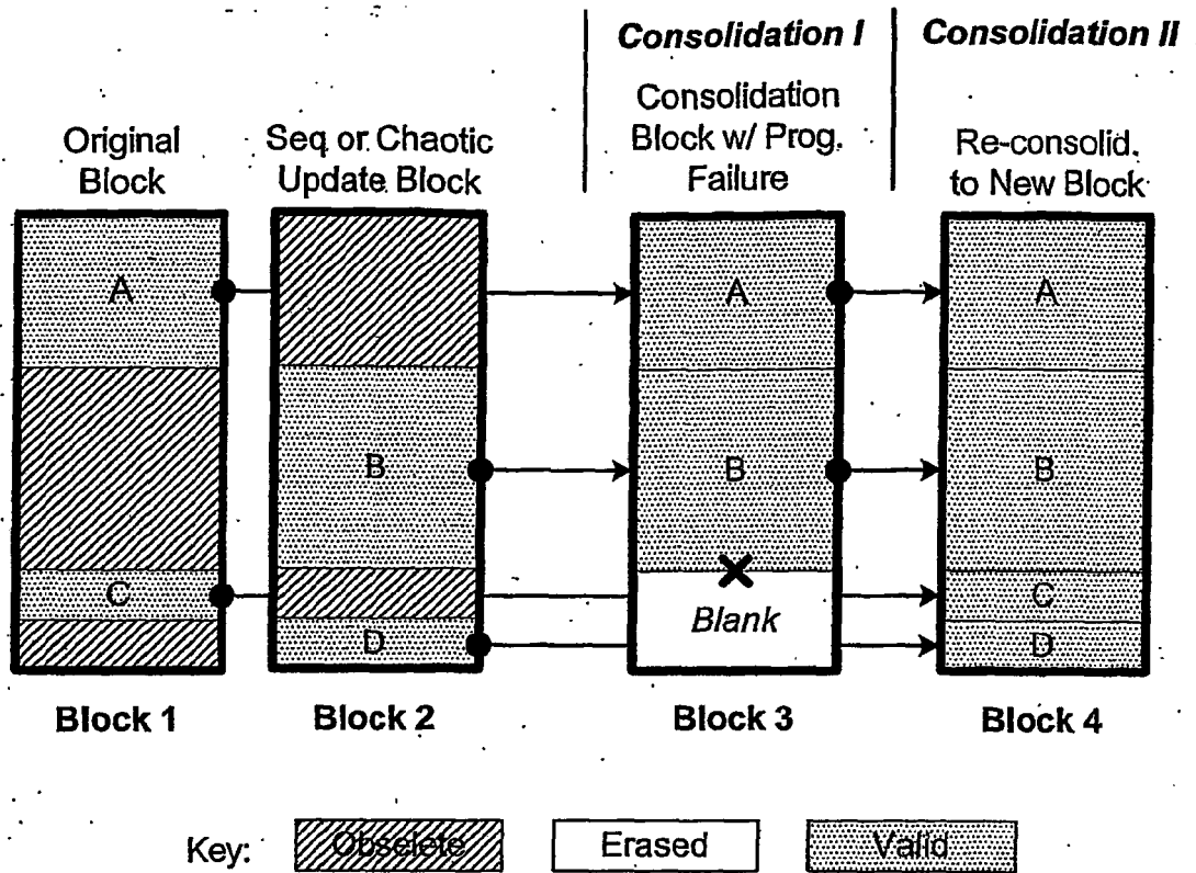
Consolidation Failure Handling by Re-consolidation
