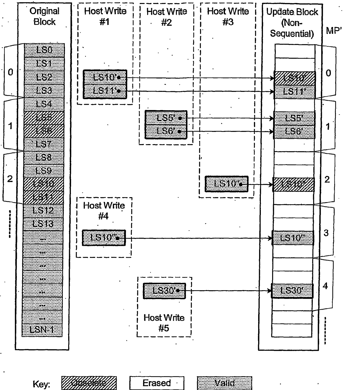
PLANE-ALIGNED CHAOTIC UPDATE (NONSEQUENTIAL) Non-Padded Example
