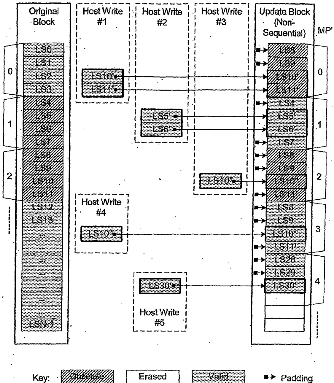
PLANE-ALIGNED CHAOTIC UPDATE (NONSEQUENTIAL) Padded Example
