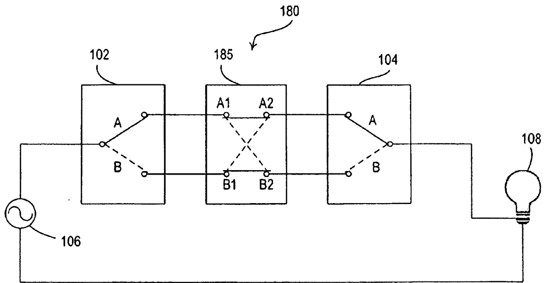
Fig. 1C Prior Art
