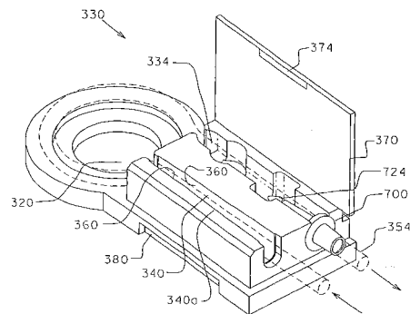
FIG. 13D
